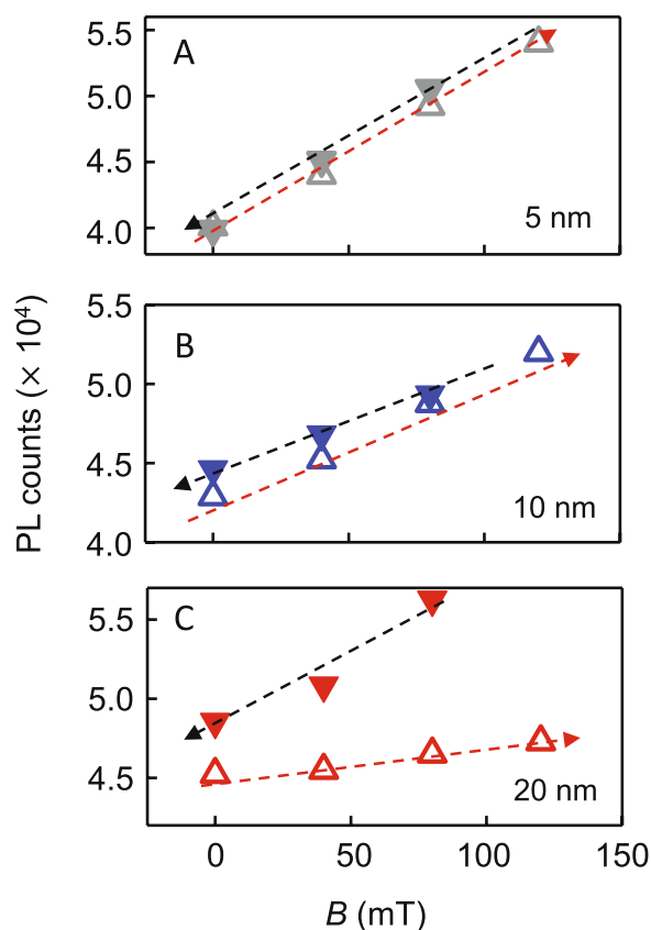
Figure 5. Integrated PL intensity for co-assemblies with (A) 5 nm MNPs, (B) 10 nm MNPs, and (C) 20 nm MNPs. Open triangles indicate magnetic field ramping up and filled triangles represent data taken while field was ramping down.
