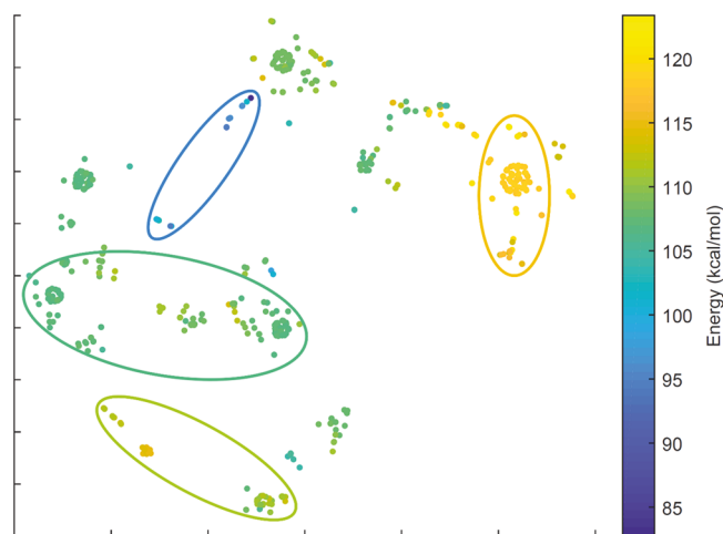
Figure 4. Clustering/categorization of C–F bond dissociation energies in various PFAS structures automatically predicted by the t-SNE machine learning algorithm. The yellow ellipse encloses C–F bonds attached to the terminal end groups of molecules and have large dissociation energies; in contrast, the blue ellipse contains C–F bonds in branched molecules and have low dissociation energies. Clusters enclosed by the lime green ellipse are associated with C–F bonds adjacent to the terminal carbon of the molecule, whereas clusters enclosed by the teal green ellipse arise from C–F bonds in the middle of the molecular chain.
