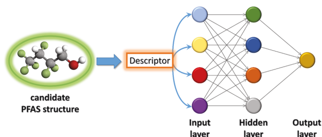
Figure 2. Schematic of the Feed-forward Neural Network used to predict PFAS bond dissociation energies in this work. PFAS bond descriptors are used in the input layer, which is subsequently processed by a hidden layer to learn a (nonlinear) mathematical mapping for generating predicted PFAS bond dissociation energies at the output layer.
