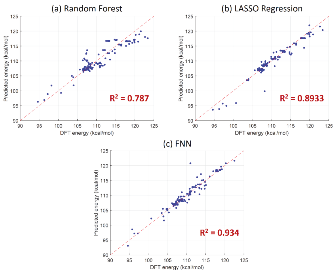
Figure 3. Comparison of the accuracy among the (a) Random Forest, (b) LASSO Regression, and (c) FNN machine learning algorithms for predicting C–F bond dissociation energies in the PFAS test set. The diagonal line in each panel represents a perfect match between that particular machine learning algorithm and the corresponding reference DFT data.
