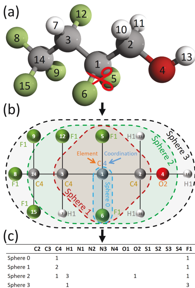
Figure 1. Schematic of the chemical descriptors and data used by our machine learning algorithms to autonomously and rapidly process C–F bond dissociation energies in general PFAS structures. Panel (a) depicts a specific target C–F bond to be dissociated, and panel (b) shows the atom labeling scheme and spheres used to construct the point descriptor table in panel (c). It is important to note that the 3D and 2D structures in panels (a) and (b) are shown only for illustrative purposes and are not used by our machine learning algorithms, whereas the simple pair descriptor table in panel (c) encodes the actual data that is used by the machine learning algorithms in this work.
