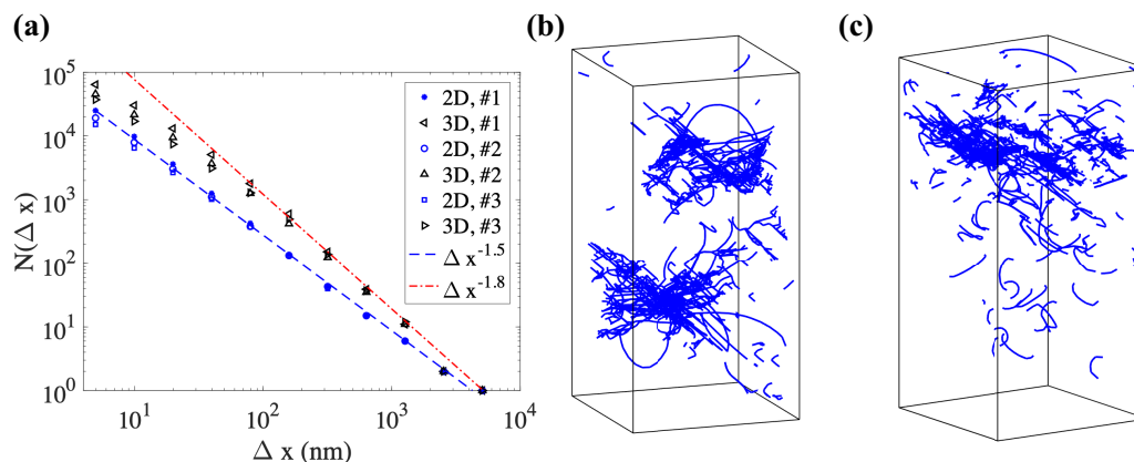
Figure 3. (a) Insensitivity of the fractal dimension of dislocation structure in irradiated Fe pillar with diameter 1500 nm, (b) dislocation configuration #2, (c) dislocation configuration #3.
