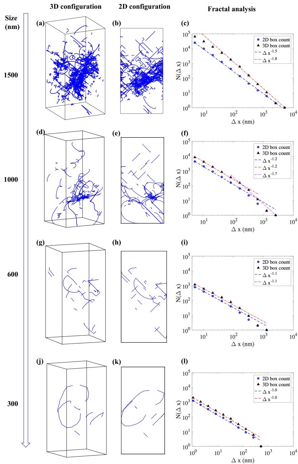
Figure 2. Effect of size and dimension on the fractal analysis of dislocation structure for irradiated Fe pillar with diameter (a–c) 1500 nm (d–f) 1000 nm, (g–i) 600 nm, (j–l) 300 nm.
