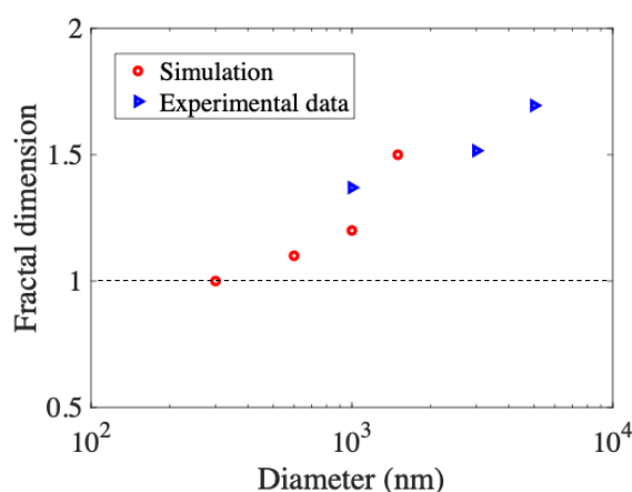
Figure 4. Size effect on the fractal dimension of dislocation microstructure. Experimental data are obtained from [16].
