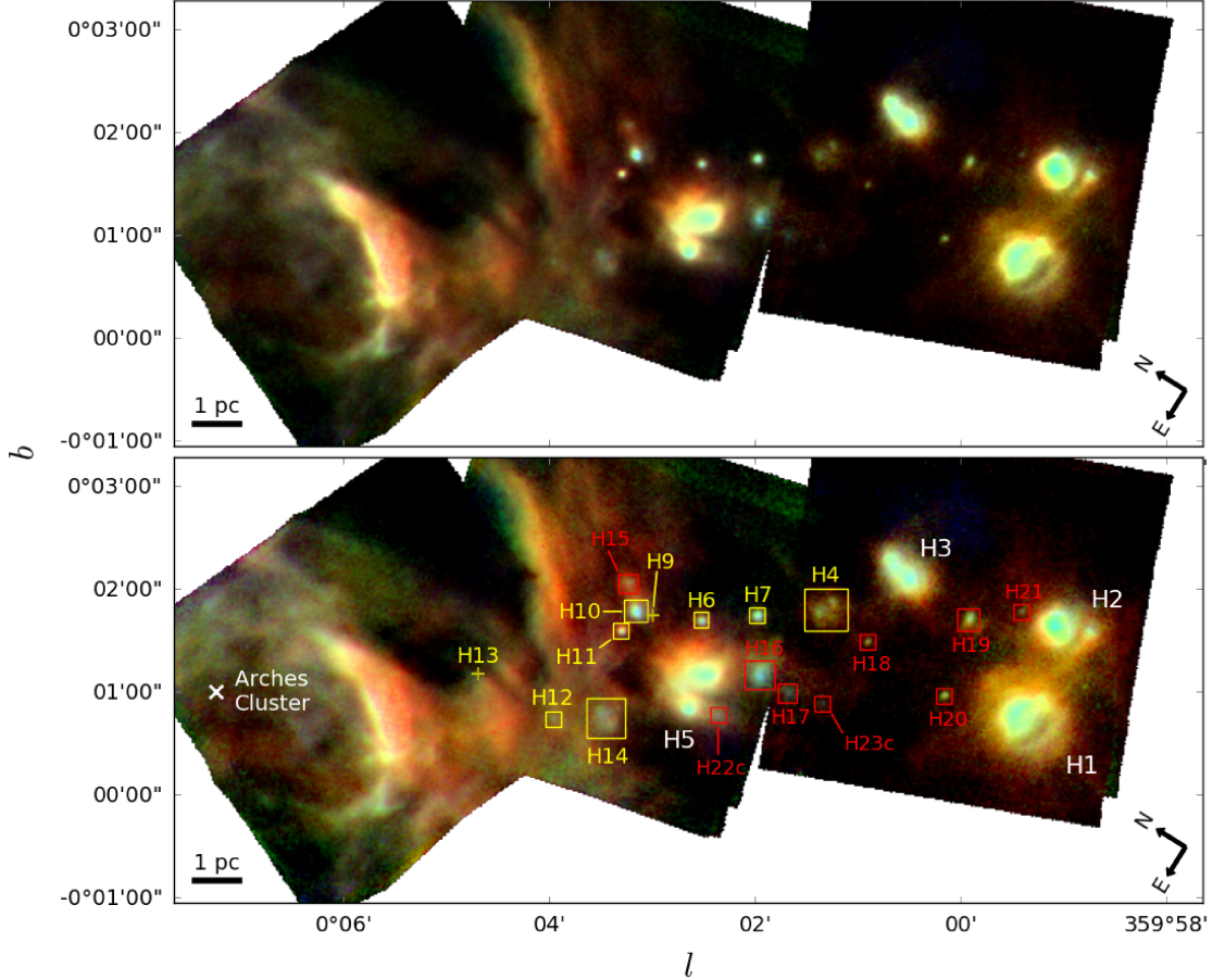
Figure 1. Top: False-color map of the H II Regions created with SOFIA/FORCAST observations at 19.7 (blue), 25.2 (green), and 37.1 \mu\text{m} (red). Bottom: A second RGB map created with the same data at a different stretch. Sources within the map are grouped into three categories which are indicated by the color of their labels. The spatially extended HII regions (H1, H2, H3, and H5) are shown in white. Additional HII regions in the complex, including H4, H6, H7, H10, H11, H12, and H14, are shown in yellow. The known sources H9 and H13 are not detected by FORCAST though their positions are indicated with a '+'. A number of additional infrared sources (H15 - H23) were also identified in the maps and are shown in red. Two of the sources (H22c and H23c) are listed as candidates because they are only detected in a single FORCAST band. The white cross denotes the location of the Arches cluster.
