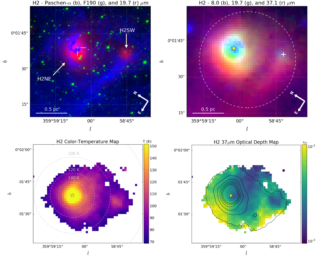
Figure 3. Top Left: False-color image of H2 with HST Paschen- \alpha (blue), HST F190 (green), & SOFIA/FORCAST 19.7 \mu\text{m} (red). P35, the candidate ionizing source of H2, is visible in the F190 map and its position is indicated by the white crosshairs. The locations of the two components H2NE and H2SW are also indicated. A scale bar and cardinal directions in equatorial coordinates are shown in the bottom left and right, respectively. Top Right: False-color image of H2 with Spitzer/IRAC 8 \mu\text{m} (blue), SOFIA/FORCAST 19.7 \mu\text{m} (green) & 37.1 \mu\text{m} (red). The location of P114 is marked by a yellow star in this panel and the two lower panels. The location of H2SW (19.7 \mu\text{m} centroid) is marked by the white '+' and the photometric extraction area is shown by the dashed circle. Bottom Left: Color-temperature map of H2 with contours (gray dashed) denoting equilibrium temperatures based on dust heating by P35. Bottom Right: 37 \mu\text{m} optical depth map of H2 with 37 \mu\text{m} contours (ranging from 0.3 to 1.8 in increments of 0.3 Jy/pix). H2SW is not visible in the 37 \mu\text{m} contours because its emission is dominated by an extended dust filament.
