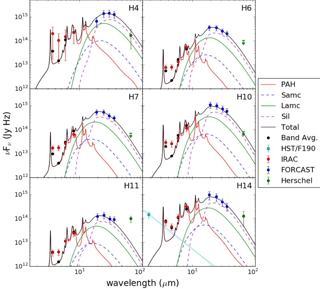
Figure 7. SED models for the remaining HII regions: H4, H6, H7, H10, H11, and H14. Details of the models are described in the text and the best-fit parameters can be found in Table 7.
