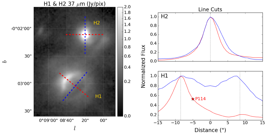
Figure 9. Line cuts through H1 & H2NE. H1 appears to have a bubble-like morphology at 37 \mu\text{m} . The apparent continuation of the bright arc-like feature into a larger bubble suggests that the shape of H1 may be generated by a density gradient in the surrounding medium. The line cuts through H1 are centered on the apparent bubble, and the location of P114 is indicated with a red star. H2NE is resolved by FORCAST, although there isn't any detailed structure is present outside of the bright central peak, which corresponds to the location of P35.
