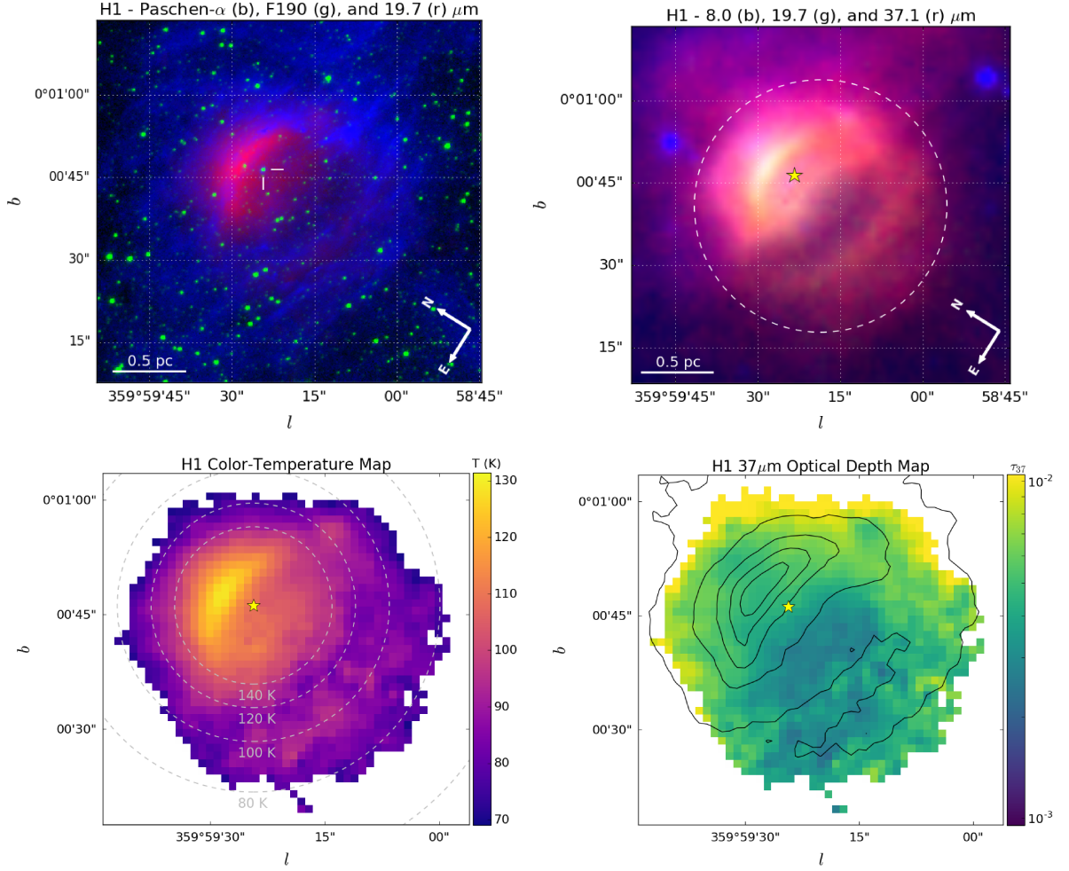
Figure 2. Top Left: False-color image of H1 with HST Paschen- \alpha (blue), HST F190 (green), & SOFIA/FORCAST 19.7 \mu\text{m} (red). P114, the candidate ionizing source of H1, is visible in the F190 map and its position is indicated by the white crosshairs. A scale bar and cardinal directions in equatorial coordinates are shown in the bottom left and right, respectively. Top Right: False-color image of H1 with Spitzer/IRAC 8 \mu\text{m} (blue), SOFIA/FORCAST 19.7 \mu\text{m} (green) & 37.1 \mu\text{m} (red). The location of P114 is marked by a yellow star in this panel and the two lower panels. The photometric extraction area is shown with the dashed circle. Bottom Left: Color-temperature map of H1 with contours (gray dashed) denoting equilibrium temperatures based on dust heating by P114. The observed dust in H1 is consistent with being heated by P114. Bottom Right: 37 \mu\text{m} optical depth map of H1 with 37 \mu\text{m} contours (ranging from 0.3 to 1.5 Jy/pix in increments of 0.3).
