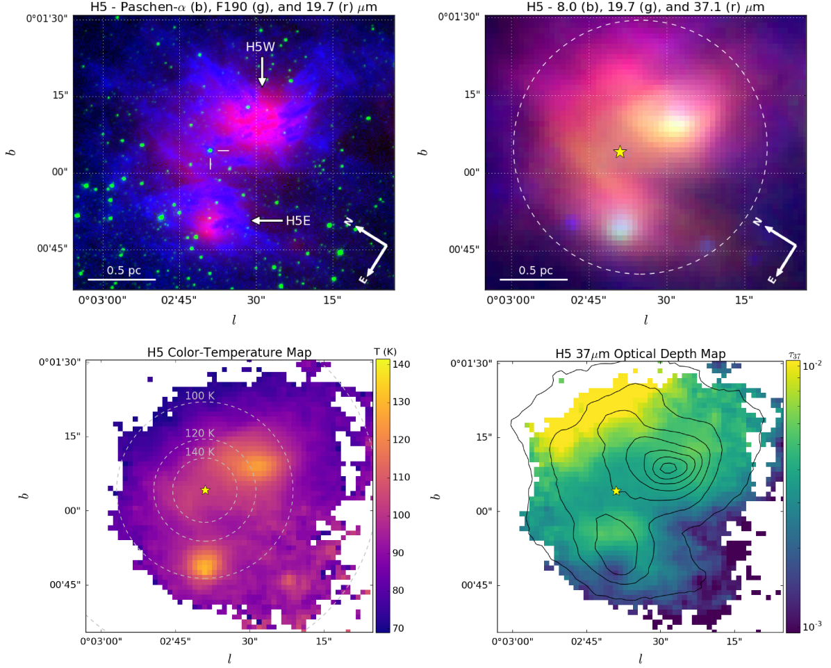
Figure 5. Top Left: False-color image of H5 with HST Paschen- \alpha (blue), HST F190 (green), & SOFIA/FORCAST 19.7 \mu\text{m} (red). P107, the candidate ionizing source of H5, is visible in the F190 image and is indicated by the perpendicular white lines. The locations of the components H5E and H5W are also indicated. Top Right: False-color image of H5 with Spitzer/IRAC 8 \mu\text{m} (blue), SOFIA/FORCAST 19.7 \mu\text{m} (green) & 37.1 \mu\text{m} (red). The location of P114 is marked by a yellow star in this panel and the two lower panels. The photometric extraction area is shown by the dashed circle. Bottom Left: A color-temperature map of H5 with contours (gray dashed) denoting equilibrium temperatures based on dust heating by P107; we suggest that this star is unlikely to be the heating source (see section 4.4). Bottom Right: A 37 \mu\text{m} optical depth map of H5 with 37 \mu\text{m} contours (ranging from 0.2 to 1.4 in increments of 0.2 Jy/pix).
