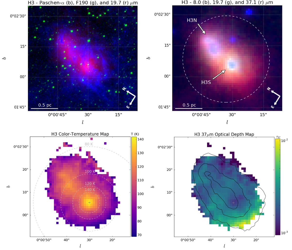
Figure 4. Top Left: False-color image of H3 with HST Paschen- \alpha (blue), HST F190 (green), & SOFIA/FORCAST 19.7 \mu\text{m} (red). The ionizing source of H3 has not been identified in previous works and its heating source is similarly unknown. Top Right: False-color image of H3 with Spitzer/IRAC 8.0 \mu\text{m} (blue), SOFIA/FORCAST 19.7 \mu\text{m} (green) & 37.1 \mu\text{m} (red). The components of H3, south (H3S) and north (H3N), are indicated on the map. The photometric extraction area is shown by the dashed circle. Bottom Left: A color-temperature map of H3. Because a probable heating source of H3 is unknown, we assume that it is located at the position of the observed temperature maximum (indicated by the grey ‘+’) and the radial temperature contours (gray dashed) have been positioned accordingly. Bottom Right: A 37 \mu\text{m} optical depth map of H3 with 37 \mu\text{m} contours (ranging from 0.3 to 0.9 in increments of 0.3 Jy/pix).
