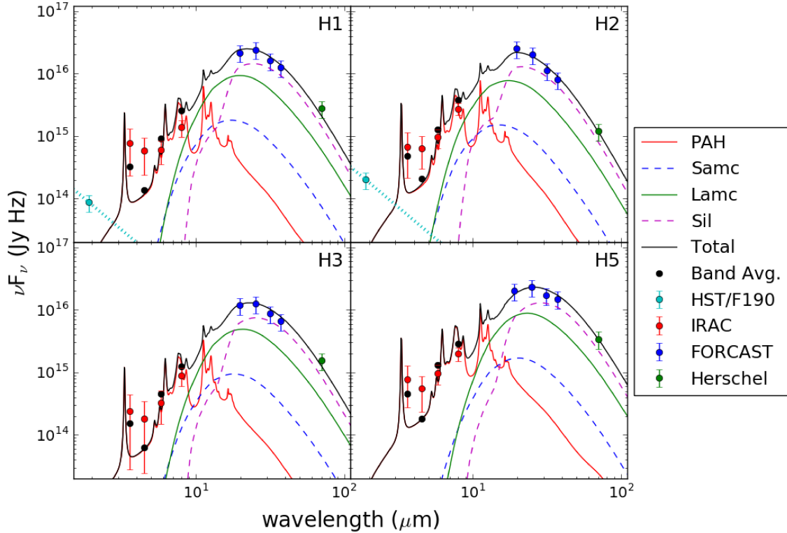
Figure 6. SED models of the HII regions H1, H2, H3, and H5. Details of the models are described in the text and the best-fit parameters can be found in Table 7.
