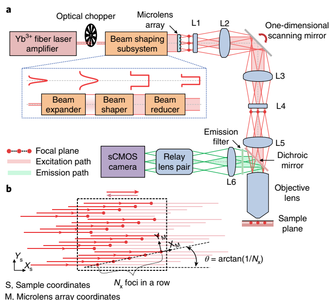
Fig. 1 | Microscope design. a , A laser amplifier beam (1,030 nm, ~280 fs pulse duration) passes through a chopper synchronized to the triangle-wave laser-scanning pattern (Supplementary Figs. 1 and 2) and is given uniform intensity across a microlens array (lenslet spacing, 100 \mu\text{m} ), which creates N_x \times N_y beamlets of equal intensity. N_x \times N_y is the number of lines scanned in the specimen. Compound (L1 and L4) and aspherical lenses (L2, L3 and L5) establish intermediate and specimen focal planes (red dots, beamlet foci) as Fourier-conjugates to the plane of the scanning mirror. Fluorescence returns through the objective lens, reflects off a dichroic mirror, and is focused by a tube lens (L6) and a relay lens pair onto a sCMOS camera synchronized to the scanning mirror. Excitation and emission pathways for three example foci are shown in red and green, respectively. Inset, the bottom shows the beam shaper, which comprises an expander, a flattop shaper and a reducer. The top shows beam intensity profiles at each stage. b , To scan images at rates \leq 1 kHz, the N_x \times N_y beamlet array is projected onto the specimen at an angle, \theta = \tan^{-1}(1/N_x) , between the (X_s, Y_s) camera-frame coordinate system (dashed rectangle) and the (X_M, Y_M) microlens array coordinate system. We generally used \leq 20 \times 20 laser foci (15 \mu\text{m} spacing between beams) oriented 2.9^\circ to the scanning direction, yielding 0.75 \mu\text{m} between scanned lines. We cropped the illumination to match the area projected onto the camera.
