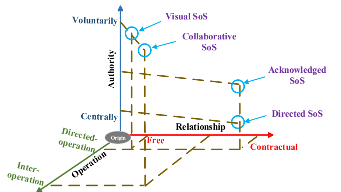
Fig. 3. Different types of SoSs
