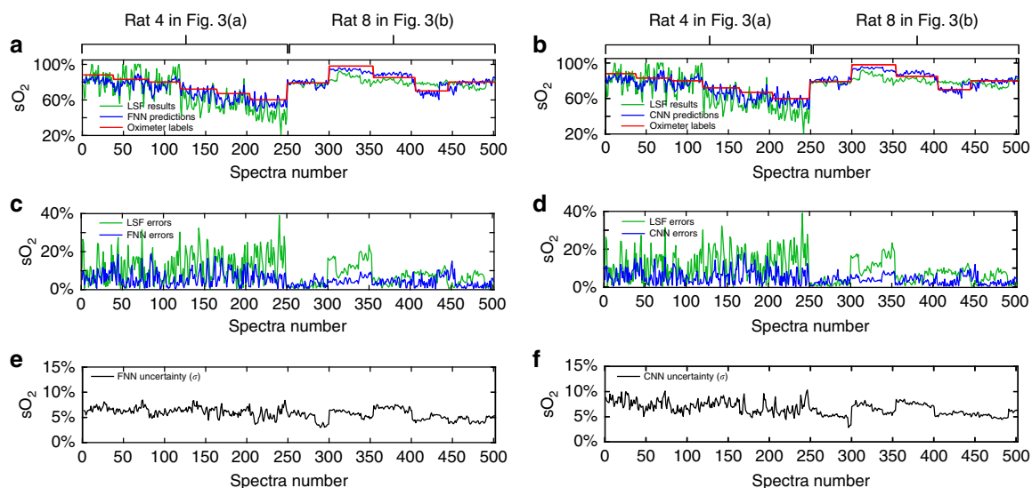
Fig. 4 Rat retinal arteriolar sO_2 of the testing data under different ventilation conditions predicted by the FNN, CNN, and LSF models. sO_2 predicted by the FNN a and CNN b , compared with the oximeter spO_2 readings and LSF calculations. Errors of sO_2 predicted by the FNN c and the CNN d model compared to the LSF results. Predicted uncertainties of sO_2 obtained by the FNN e and the CNN f model measured by the standard deviations ( \sigma ). The first 248 spectra were from ref. 13, and the rest were from ref. 15.
