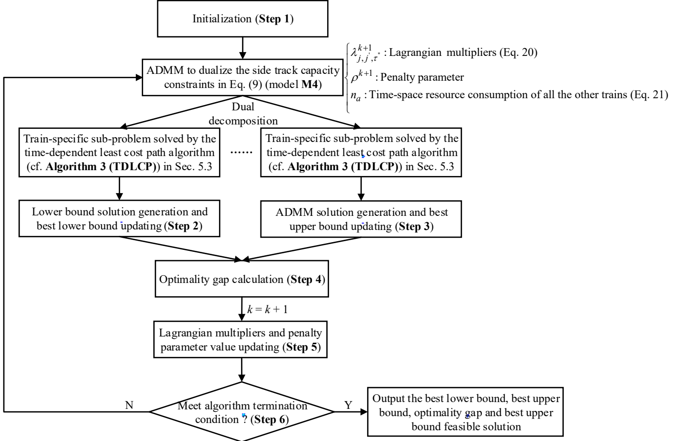
Fig. 4. ADMM-based solution framework for iteratively updating of the best lower and upper bounds (cf. Algorithm 1 (ADMM) )
