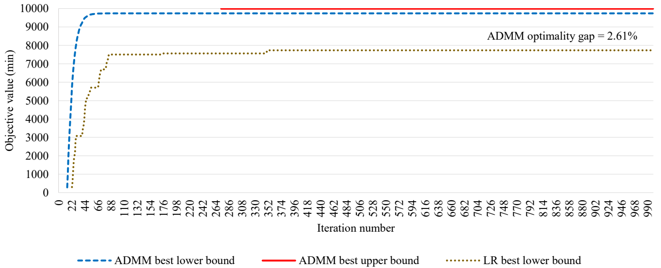
Fig. 9. Best lower bound and upper bound values of ADMM and LR for the scenario 9 with iteration number (28 lines, 30 trains)
