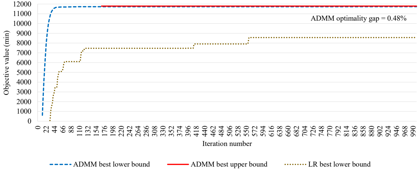
Fig. 10. Best lower bound and upper bound values of ADMM and LR for the scenario 12 with iteration number (34 lines, 36 trains)
