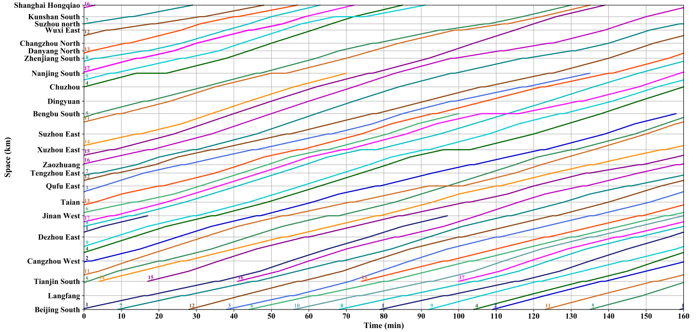
Fig. 11. Cyclic train diagram for scenario 4 obtained by ADMM with 17 lines and 18 trains (the numbers above the lines are the line numbers)
