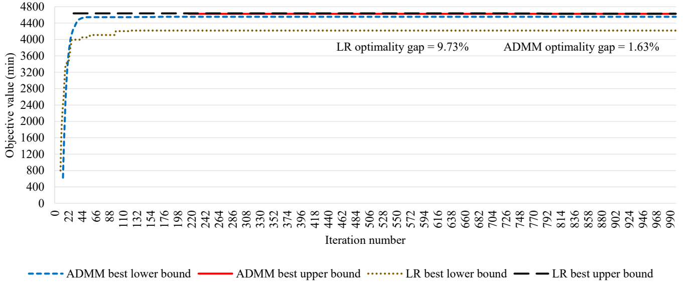
Fig. 8. Best lower bound and upper bound values of ADMM and LR for the scenario 4 with iteration number (17 lines, 18 trains)
