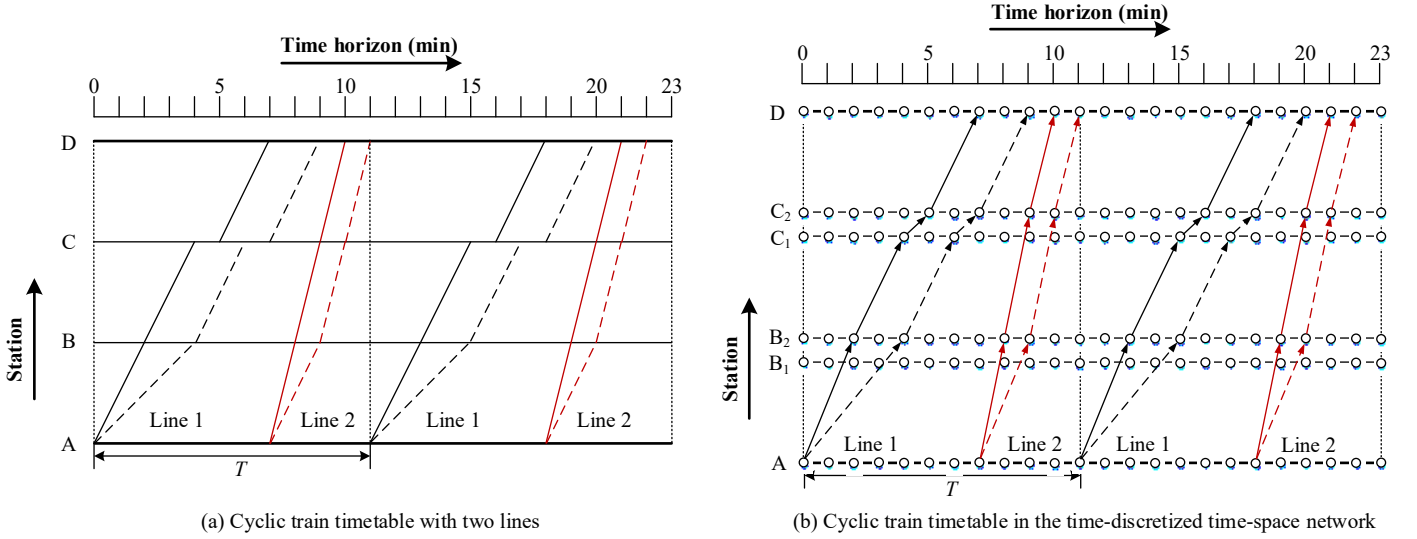
(a) Cyclic train timetable with two lines (b) Cyclic train timetable in the time-discretized time-space network Fig. 2. Expression of the cyclic train timetable with variable trip times in the time-discretized time-space network
