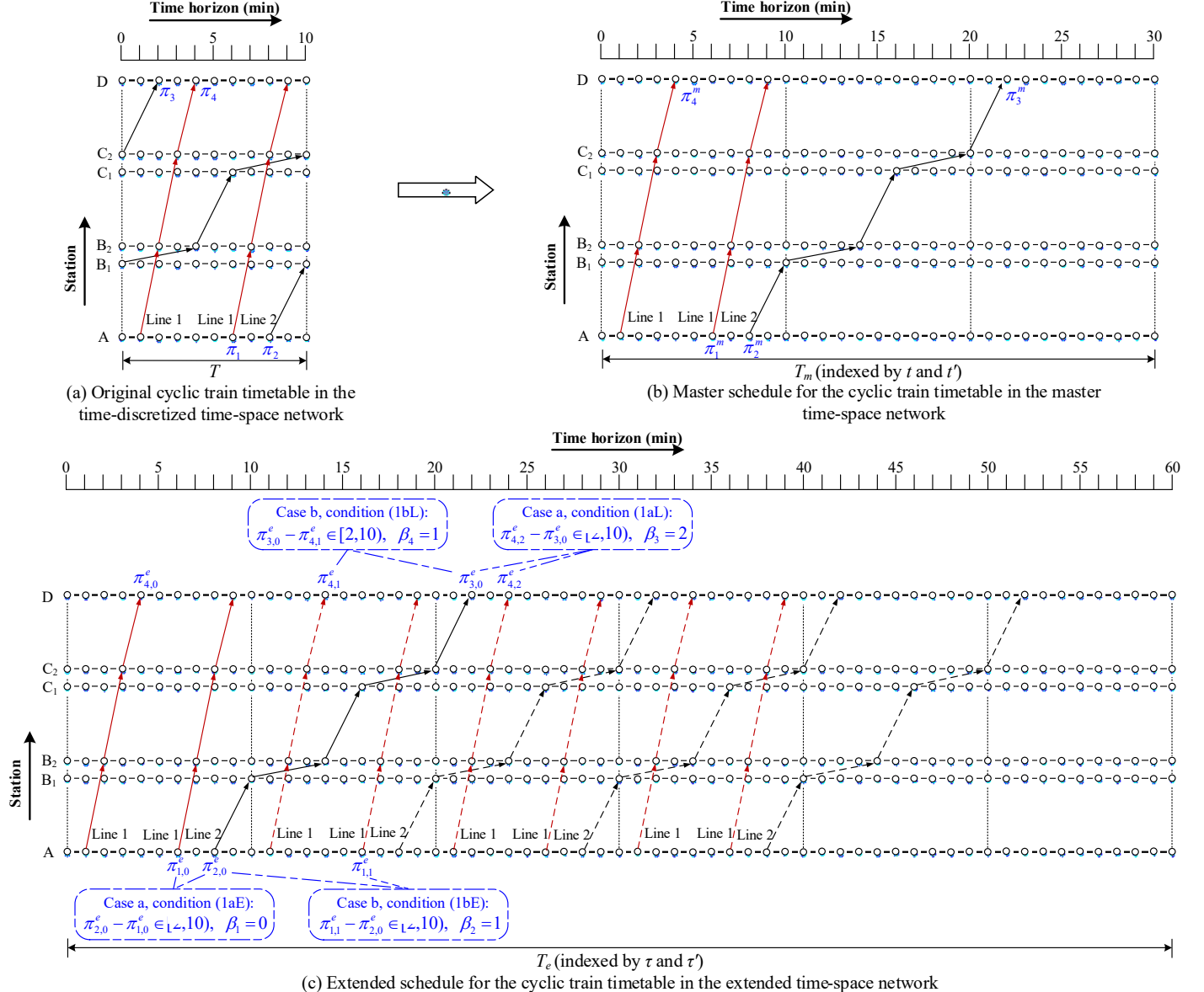
Fig. 3. Transformation of the original cyclic train timetable into the master and extended schedules
