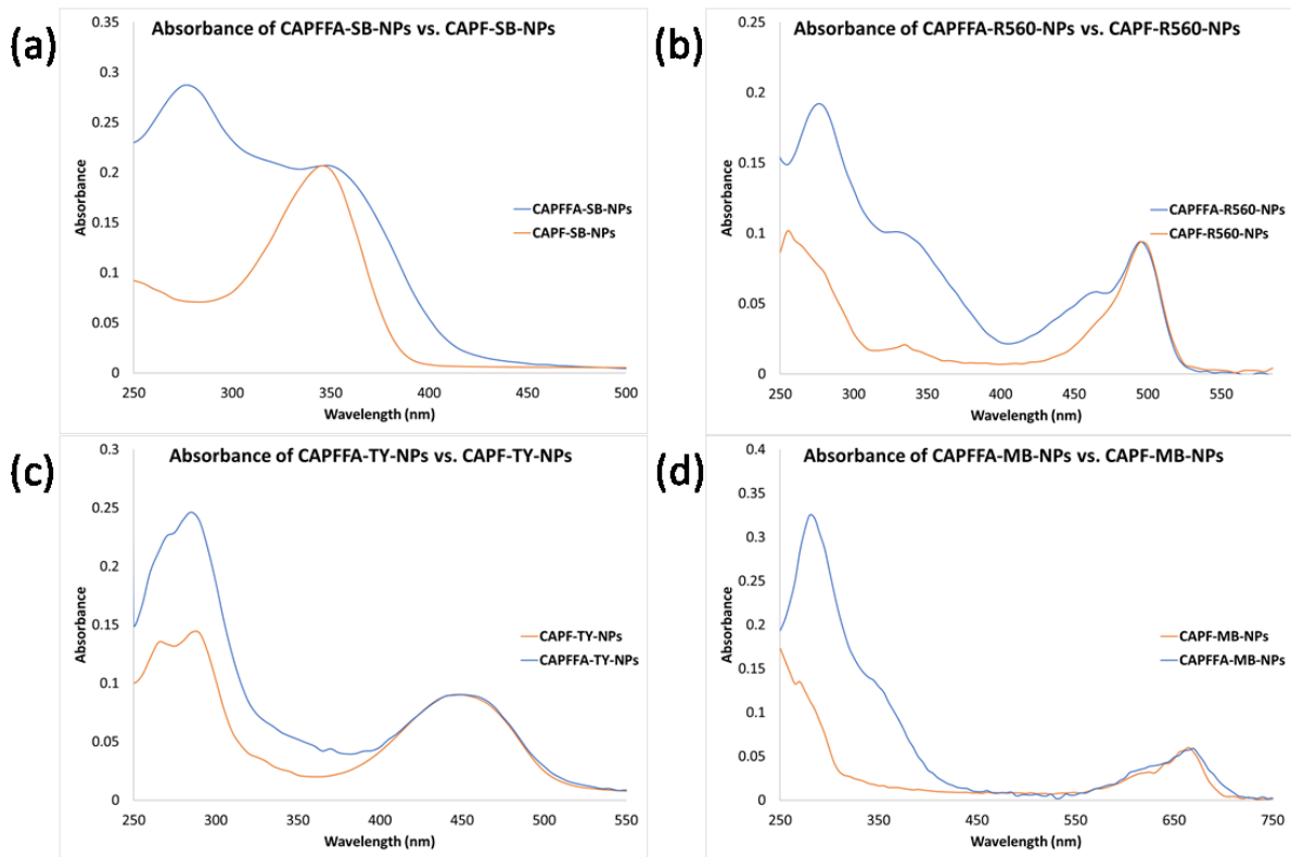
Fig. 4. Absorbance spectra (a) of Stilbene 420, (b) Rhodamine 560, (c) Tracer Yellow, and (d) Methylene Blue encapsulated particles, PEGylated (orange curve) and folate-conjugated (blue curve). All spectra have been normalized to the specific encapsulated dye peak of each particle.
