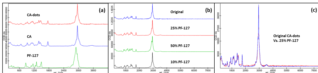
Fig. 2. Raman spectra of individual components and nanoparticles are shown in (a). Raman spectra of nanoparticles of varying compositions (10-50% by weight PF127) were simulated from component spectra and evaluated to fit the original CA-dot spectra in (b). Examples of
