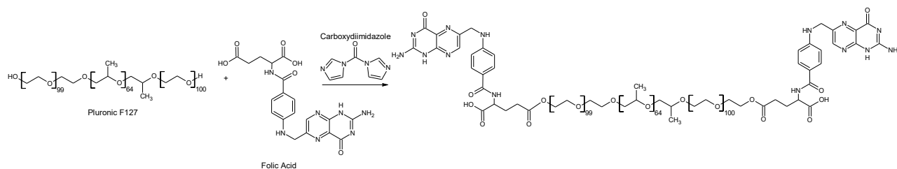
Fig.1. Conjugation scheme of folic acid and PF127 copolymer.
