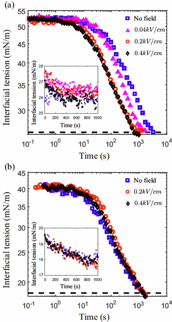
FIG. 2. Dynamic interfacial tension for (a) 4 \mu\text{M} OLOA 11000 in Isopar-M and (b) 10 \mu\text{M} Pluronic L64 in 100 cSt silicone oil. The dashed line represents the steady-state interfacial tension. Inset: Dynamic interfacial tension for each system during the last 1000 s under each electric field. The time axis has been shifted so that all the curves fit in the same time range of 0 to 1000 s.
