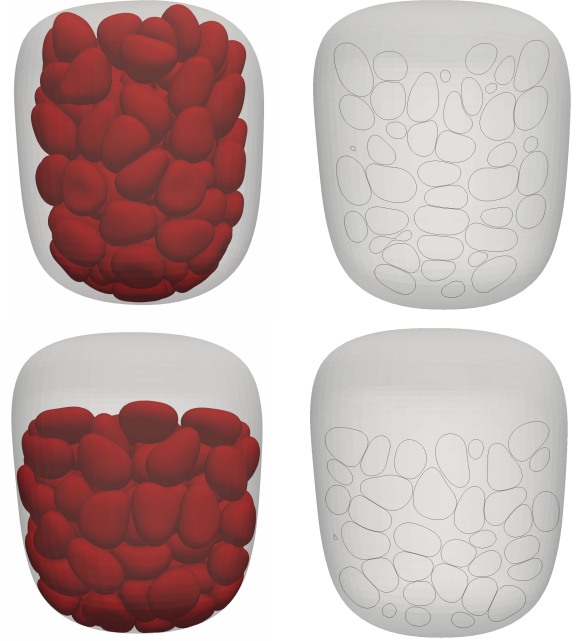
Figure 7: Shown is a high-volume fraction sedimentation due to gravitational force. The initial configuration (top figures) has a volume fraction of 47%. As the cells sediment to the lower part of the domain (bottom figures), the local volume fraction of the final state in this lower part of the domain is around 55%. Shown on the right side are slices through the center of the domain together with the RBC boundaries in the initial and final configuration. The full simulation video is available at https://vimeo.com/329509435 .
