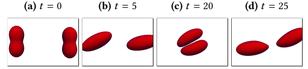
Figure 10: Snapshots of two vesicles in shear flow.
