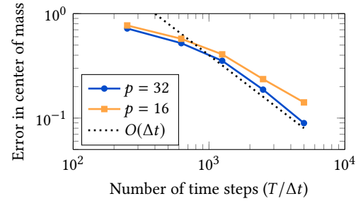
Figure 11: Shown is the error in the final ( T = 25 ) centroid location as we decrease the time step size for two spherical harmonic orders 16 and 32. We observe O(\Delta t) convergence in time and hence the collision detection algorithm converges at the same order as the time stepper.
