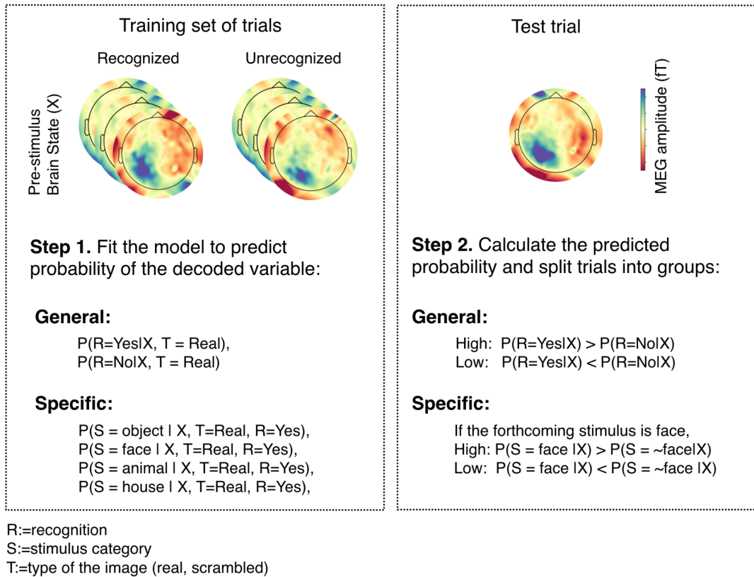
Supplementary Figure 3. Schematics of probability groups split according to the General and Specific models. Step 1: We fit the weights of the logistic regression decoder using a training set of trials. For the General model we used real-image trials to decode the recognition report (yes/no). For the Specific model we used real-image trials that were recognized to decode the stimulus category. Step 2: Using the fitted logistic regression decoder from step 1, we calculate the probability of the decoded variable for each single test trial. For the General model, the trial will be placed in the high-probability group if the logistic regression model predicts that it is more likely to be recognized than unrecognized. For the Specific model, the trial will be placed in the high-probability group if the logistic regression model predicts the forthcoming stimulus category with a probability that is higher than that of every other category. Note, there is no overlap between trials used in the two steps.
