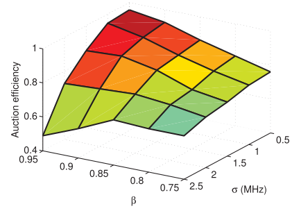
Fig. 6. Auction efficiency under different confidence level \beta and spectrum standard deviation \sigma .
