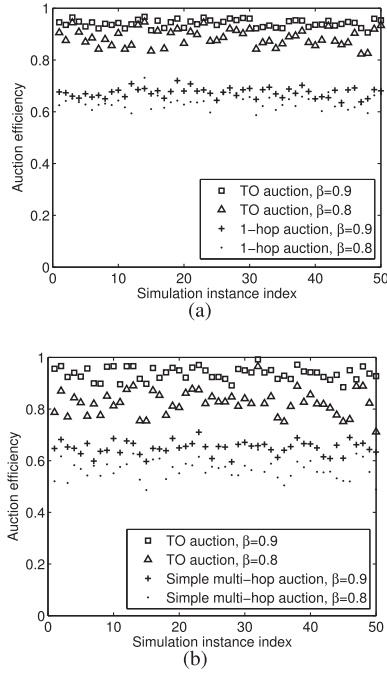
Fig. 5. Auction efficiency comparison with a 1-hop auction scheme and a simple multi-hop auction scheme. (a) Single-hop data transmission scenario. (b) Multi-hop data transmission scenario.
