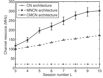
Fig. 3. Spectrum resources utilized by the three different architectures.
