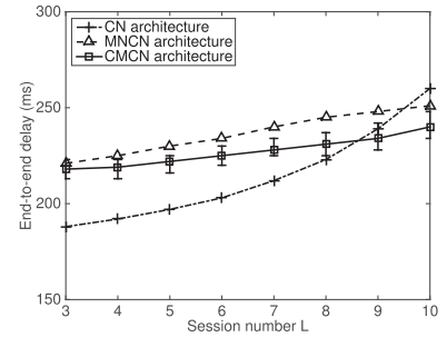
Fig. 4. End-to-end delay comparison among three architectures.
