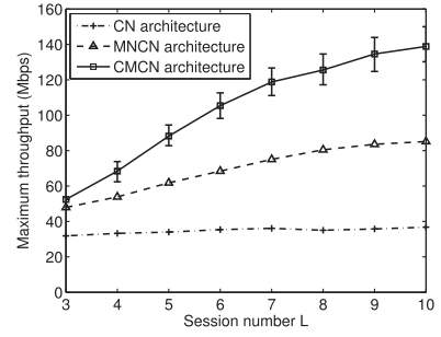
Fig. 2. Maximum throughput comparison among three architectures.
