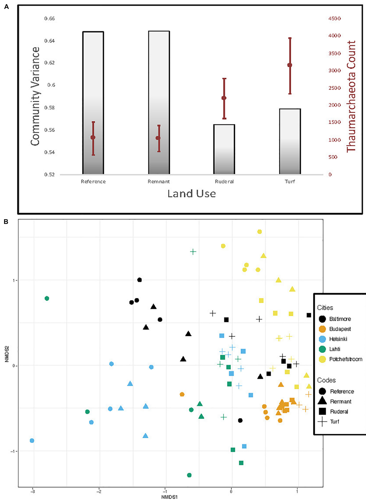
FIGURE 5 | (A) Gray bars show variance in amplicon-based archaeal communities and overlaid in red is the abundance of sequences matching Thaumarchaeota. (B) NMDS of archaeal communities based on 16S rRNA sequencing and analysis with the dada2 pipeline.
