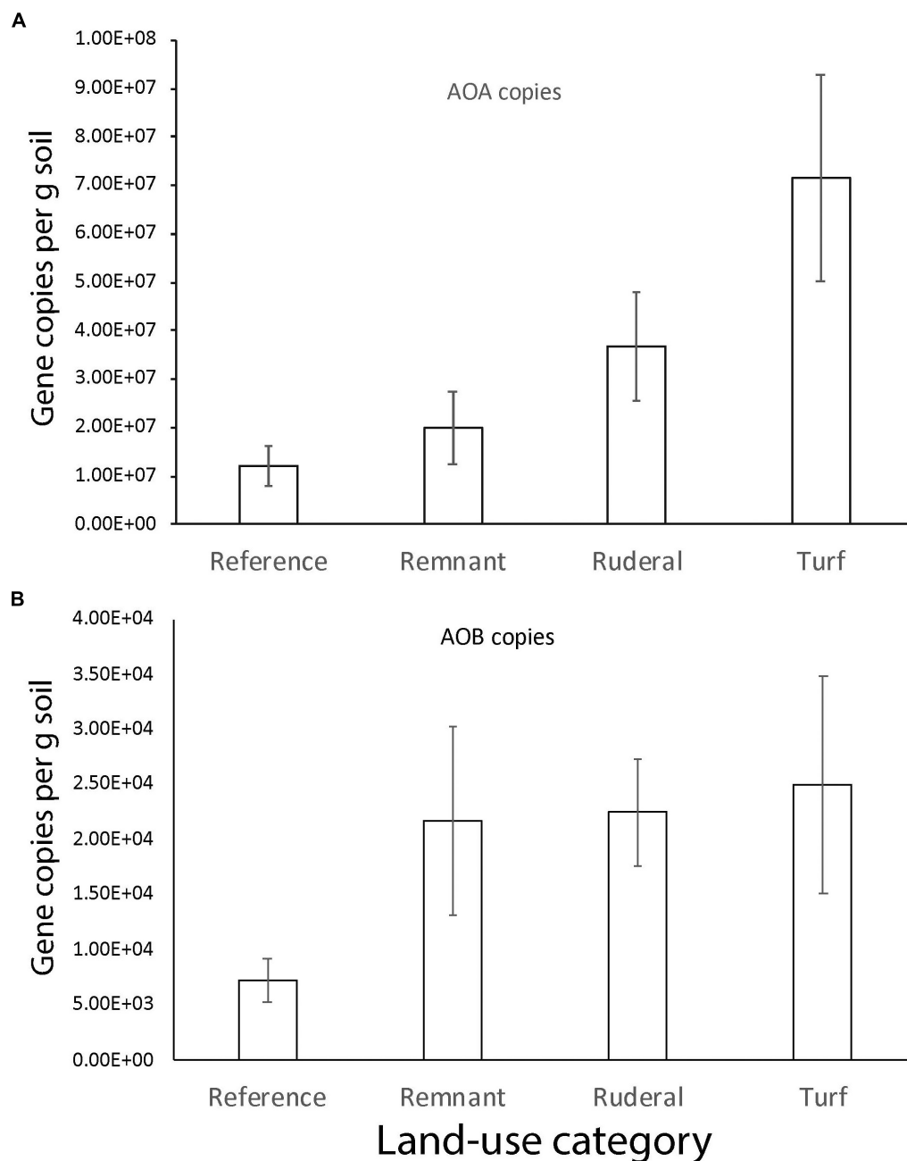
FIGURE 6 | The number of gene copies (g of soil -1 ) for (A) archaeal and (B) bacterial amoA .
