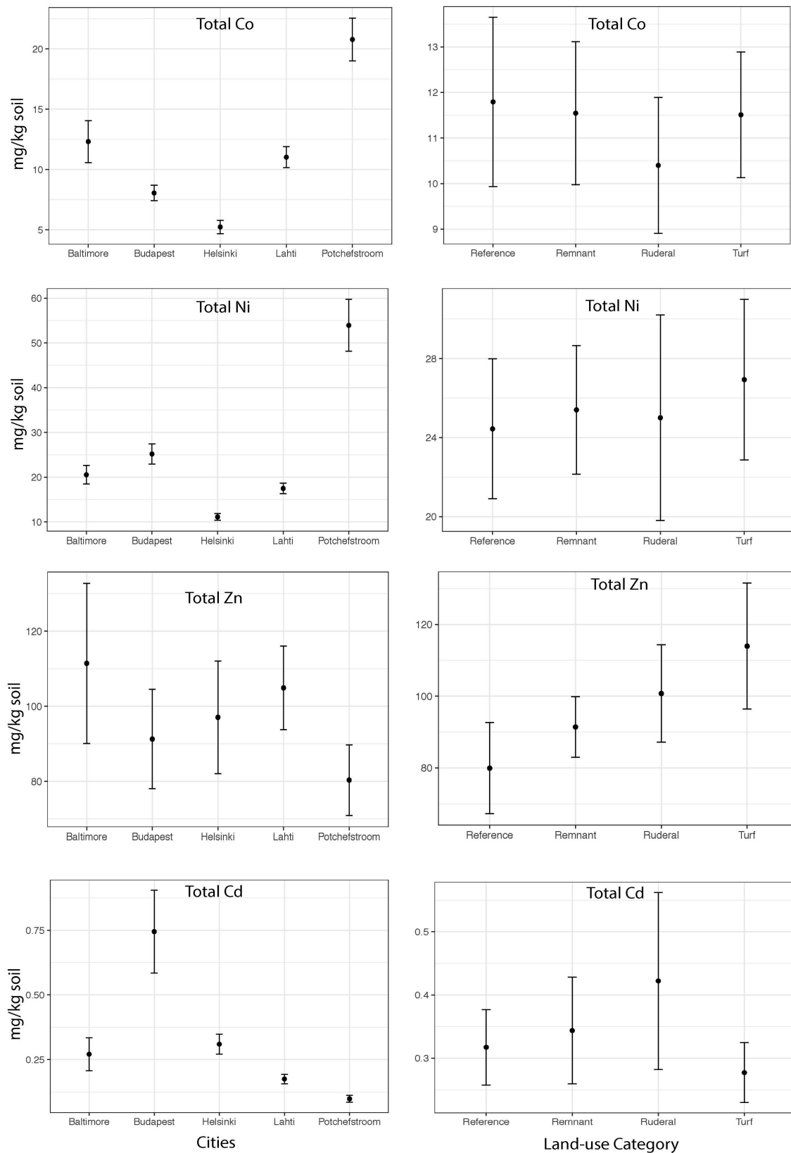
FIGURE 2 | The mean concentrations of total Co, Cd, Ni and Zn (mg of metal kg soil -1 ) within each city and the mean concentration of total Co, Cd, Ni and Zn (mg of metal kg soil -1 ) for each land-use averaged across all cities.
