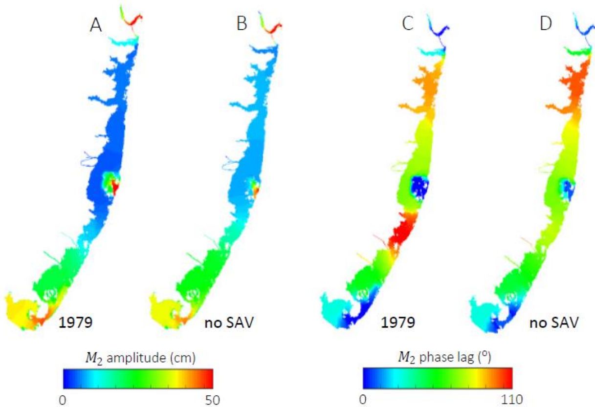
Figure 3: M_2 amplitude (cm) and phase lag ( ^\circ ) for year 1979 (a, c) and no SAV case (b, d).
