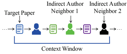
Figure 2: Example showing the behavior of skip-gram model of Camel on a sample meta-path guided random walk.
