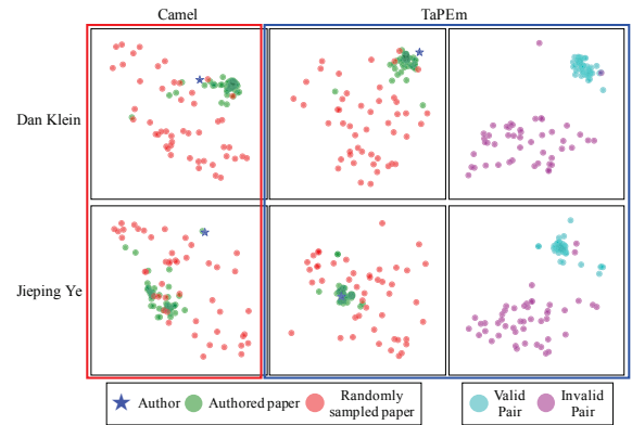
Figure 6: t-SNE visualization of author, paper and pair embeddings for two authors: Dan Klein and Jieping Ye.
