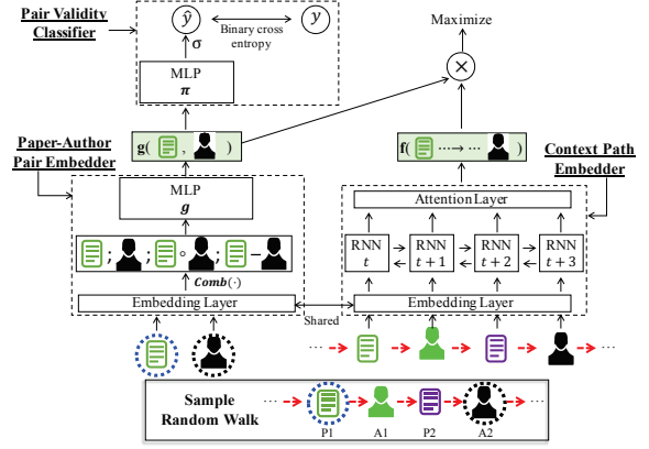
Figure 5: An overview of TaPEm.
