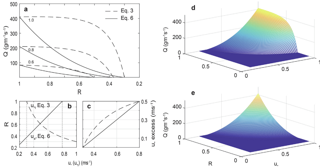
Fig. 1. Graph (a) illustrating the effect of incomplete (Eq. (3)) and complete (Eq. (6)) implementation of the drag partition R on streamwise sediment flux density Q (g m -1 s -1 ) for soil threshold wind friction velocity u_{*ts} = 0.3 m s -1 and total wind friction velocities ( u_* = u_* ) of 0.6, 0.8 and 1 m s -1 . Differences in Q responses to increasing roughness (decreasing R ) are determined by the nonlinear increase in u_{*t} with decreasing R if only adjusting u_{*ts} by R (Eq. (3)), while for Eq. (6) u_{*s} responds linearly to the adjustment of u_* by R , shown in panel (b) for u_{*ts} = 0.3 m s -1 and u_* = 0.8 m s -1 . Using the same values of R from (b), panel (c) shows that for a given reduction of u_* from 0.8 m s -1 to u_{*s} , Eq. (3) produces a nonlinear increase in excess wind friction velocity (calculated as u_* - u_{*s} ) compared to that produced by Eq. (6). Over a range of wind friction velocities and roughness densities, Q (Eq. (3)) remains large and then rapidly declines at large roughness densities (d) when it should decline with increasing roughness (e). Values of Q for (a), (d) and (e) were calculated using Kawamura (1951), with C = 2.78 , \rho_a = 1230 kg m -3 , and g = 9.8 m s -2 .
