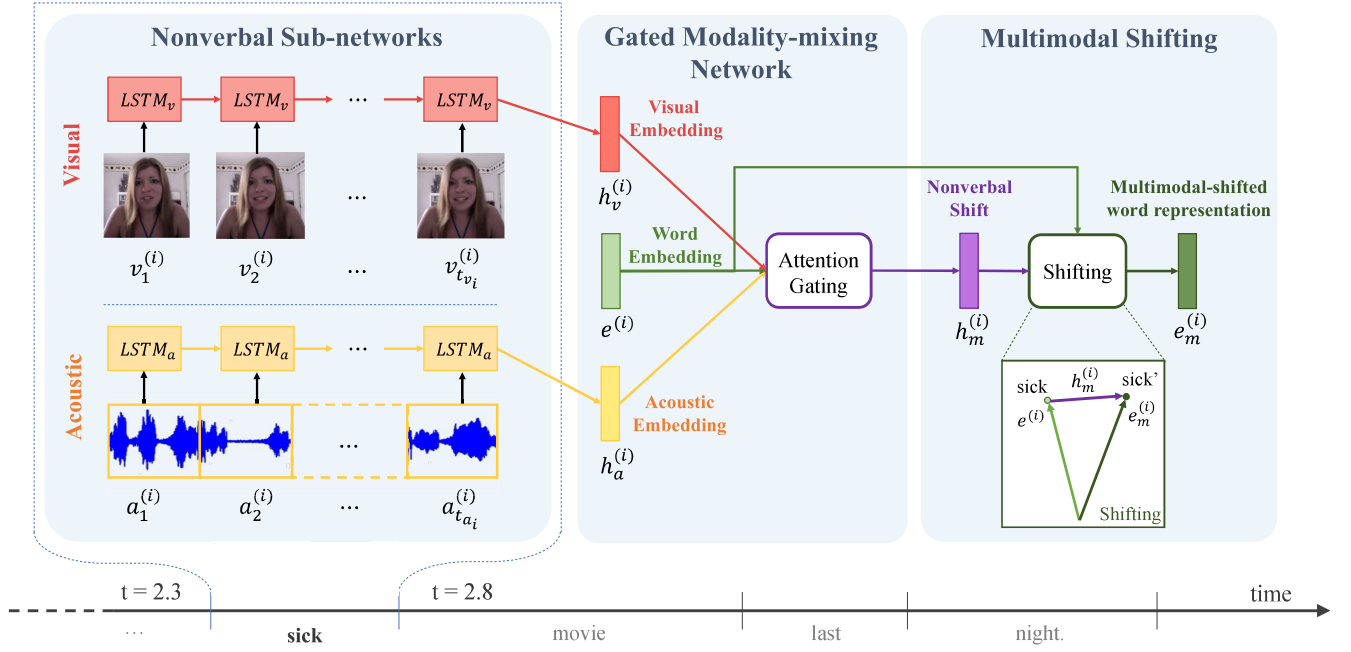
Figure 2: An illustrative example for Recurrent Attended Variation Embedding Network (RAVEN) model: The RAVEN model has three components: (1) Nonverbal Sub-networks, (2) Gated Modality-mixing Network, and (3) Multimodal Shifting. For the given word “sick” in the utterance, the Nonverbal Sub-networks first computes the visual and acoustic embedding through modeling the sequence of visual and acoustic features lying in a word-long segment with separate LSTM network. The Gated Modality-mixing Network module then infers the nonverbal shift vector as the weighted average over the visual and acoustic embedding based on the original word embedding. The Multimodal Shifting finally generates the multimodal-shifted word representation by integrating the nonverbal shift vector to the original word embedding. The multimodal-shifted word representation can be then used in the high-level hierarchy to predict sentiments or emotions expressed in the sentence.
