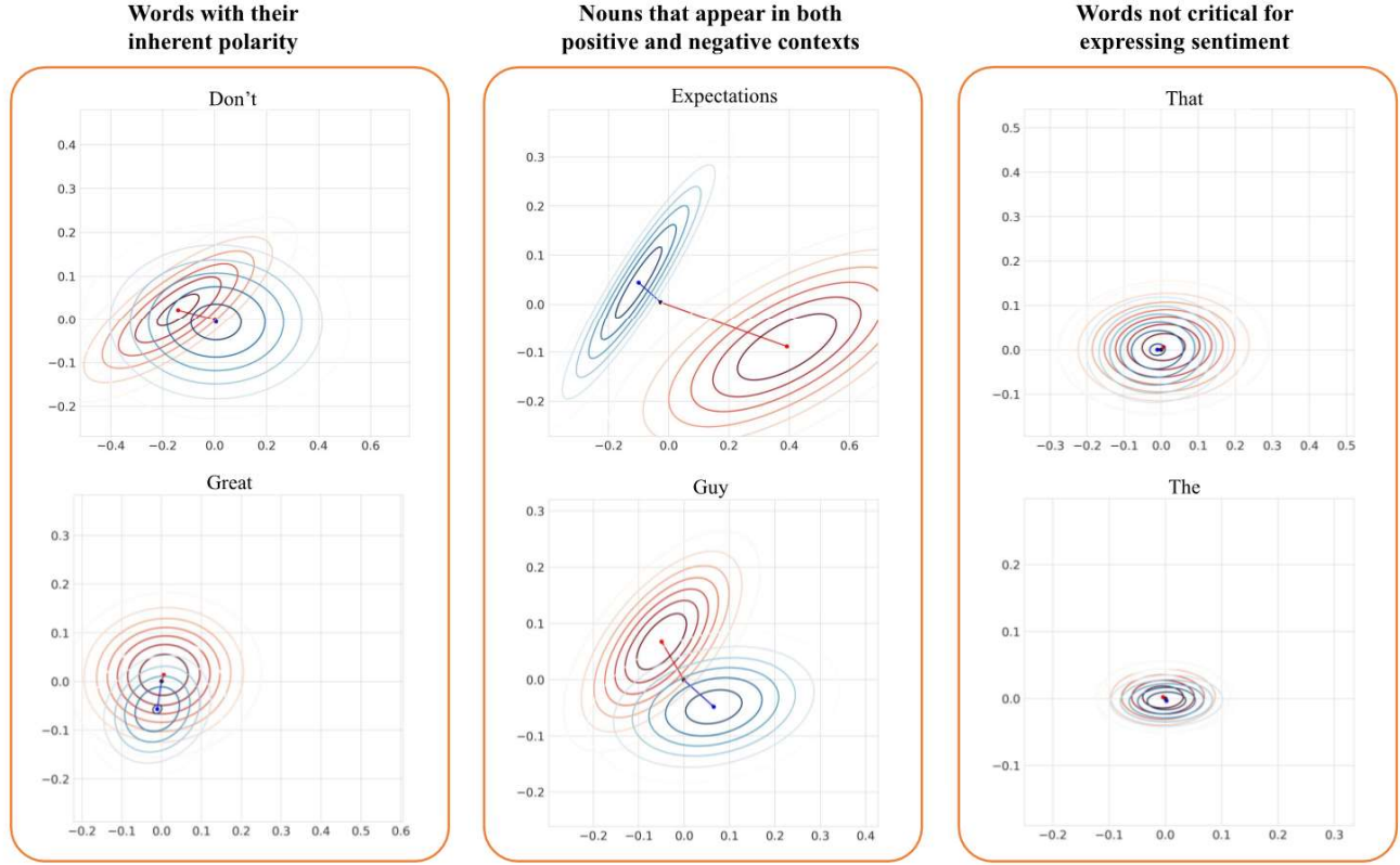
Figure 3: The Gaussian contours of shifted embeddings in 2-dimensional space. Three types of patterns observed in the distribution of all instances of the same word type: words with their inherent polarity will need a drastic variation to convey opposite sentiment; nouns that can appear in both positive and negative contexts will have large variations in both cases; words not critical for expressing sentiment minimal variations in both positive and negative contexts and the distribution of positive/negative instances significantly overlap.
