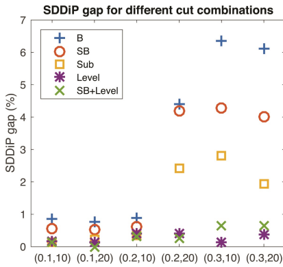
Fig. 3: SDDiP optimality gaps for different cut combinations.
