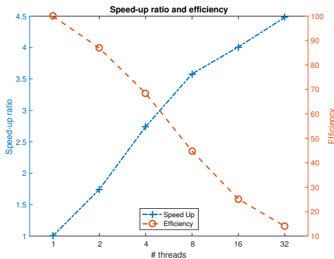
Fig. 8: Parallelization speed-up ratio & efficiency ( \mathcal{T}_{14}^{0.2,20} instance).
