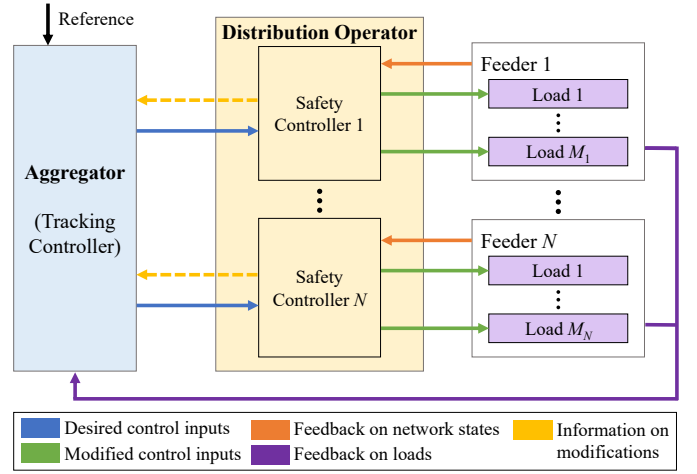
Fig. 2. Specific coordination scheme within the operator-centric framework. The aggregator calculates its desired control input based on the reference signal and feedback from loads. The operator estimates the feeders’ states based on measurements and modifies the control inputs if necessary. Information on modifications may or may not be shared with the aggregator.
