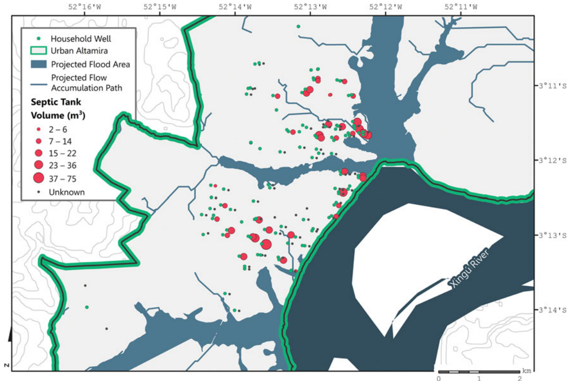
Figure 2 Location of surveyed household wells, septic tanks, projected flow accumulation paths, and projected flood areas in urban Altamira. Projected flood area source: SEMAT (2016). (Color figure available online.)
