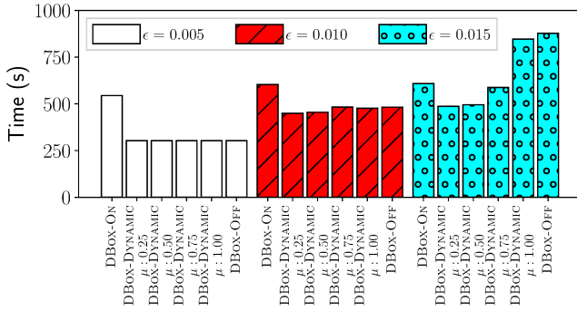
Figure 8: Response time of BPS-HDBSCAN for several DENSEBOX configurations: DBox-ON, DBox-DYNAMIC ( \mu = 0.25, 0.5, 0.75, 1 ), and DBox-OFF on the Gaia dataset with minpts = 4 , n_p = 200 , n_c = 16 , and n_{GPU} = 2 .
