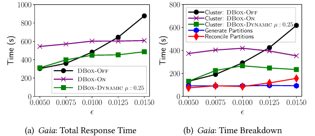
Figure 9: Response time vs. \epsilon on Gaia , where BPS-HDBSCAN is executed with n_{GPU} = 2 , minpts = 4 , n_p = 200 , and n_c = 16 . (a) Total response time; and, (b) Time breakdown.
