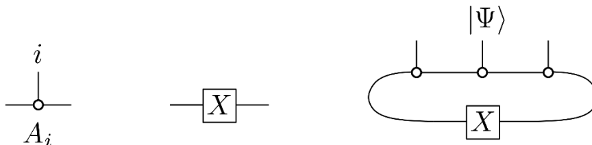
Figure 1. This figure illustrates an MPS with n = 3 physical spins, defined in terms of a family \{A_j\}_{j=1}^p of matrices and a matrix X .
