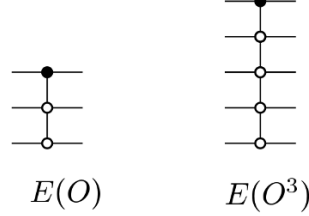
Figure 12. This figure shows the tensor network representations of E_O and E_{O^3} .
