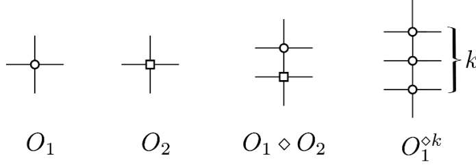
Figure 9. The product of two MPO tensors O_1 and O_2 , as well as the power O_1^{\diamond k} .
