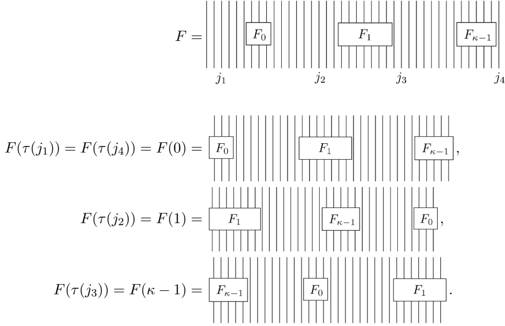
Figure 6. Example for F and sites j_1, j_2, j_3, j_4 \in \{1, \dots, n\} with \iota(j_1) = \iota(j_4) = 7 , \iota(j_2) = 19 , and \iota(j_3) = 35 .
