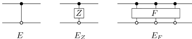
Figure 2. The transfer operator E , as well as E_Z for Z \in \mathcal{B}(\mathbb{C}^p) , and E_F for F \in (\mathbb{C}^p)^{\otimes 3} .
