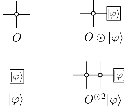
Figure 13. This figure illustrates the definition of the product O \odot |\varphi\rangle .
