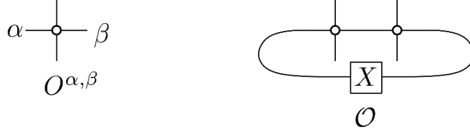
Figure 8. Alternative parametrization of an MPO \mathcal{O} .
