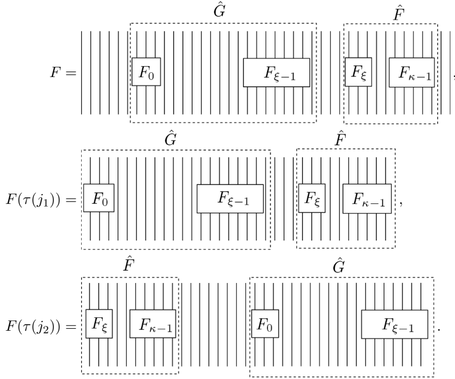
Figure 7. Example for the operator F and the corresponding F(\tau(j_1)) and F(\tau(j_2)) .
