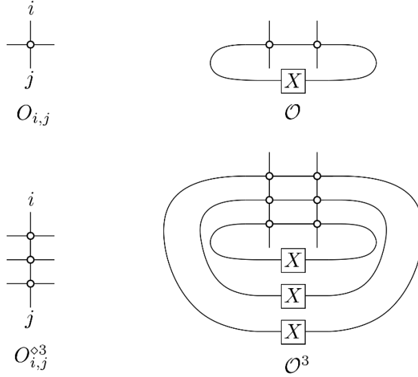
Figure 10. This figure shows an MPO \mathcal{O} = \mathcal{O}(O, X, 2) defined in terms of matrices \{O_{i,j}\}_{i,j} and the matrices \{O_{i,j}^{\diamond 3}\}_{i,j} defining the MPO \mathcal{O}^3 . Left-multiplication by an operator corresponds to stacking a diagram on top.
