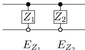
Figure 3. The product E_{Z_1 \otimes Z_2} = E_{Z_1} E_{Z_2} of two transfer operators. Left-multiplication by an operator corresponds to attaching the corresponding diagram on the left.
