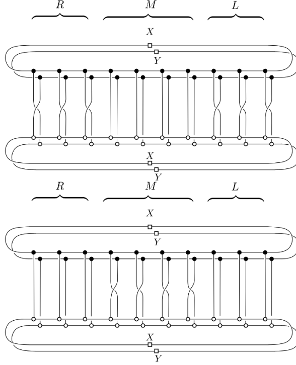
Figure 4. The two expressions in equation (5.3), where L , M and R are used to denote the sites defined in (5.2).
