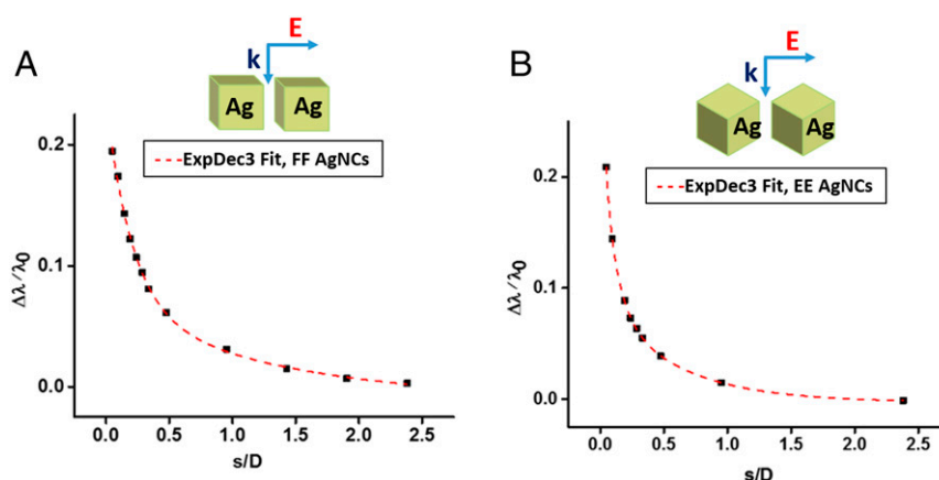
Fig. 4. Dependence of the extinction band maximum shift ( \Delta\lambda/\lambda_0 ) as a function of the interparticle separation, which is scaled by either (A) the size of the monomer for the FF AgNCs or (B) the diameter of the monomer for the EE AgNCs. The data fit well to the third-order exponential model.
