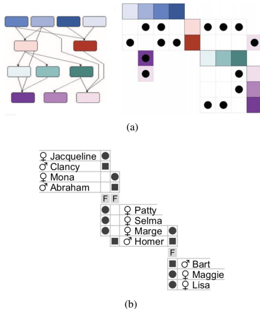
Figure 10: The quilts technique. (a) Showing how a small layered network (left) is represented using quilts (right). Links that connect nodes in nonconsecutive layers are represented by colored cells with black dots in them. (b) Simpson family as represented by a quilt [BDF*10]. © 2010 IEEE, reprinted with permission.
