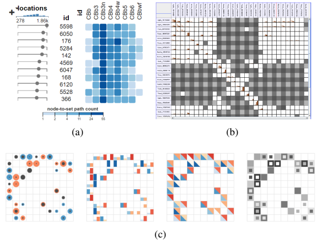
Figure 9: Adjacency matrix approaches. (a) Connectivity Matrix approach where cells represent total path counts between nodes [KLS*17]. Image courtesy of Ethan Kerzner. (b) Aggregated matrix represented by an adjacency matrix where aggregated edge attributes are displayed in the cells [EDG*08]. © 2008 IEEE, reprinted with permission. (c) Comparison of on-edge encoding to adjacency matrix edge attribute encodings [ABHR*13]. © 2013 ACM, reprinted with permission.
