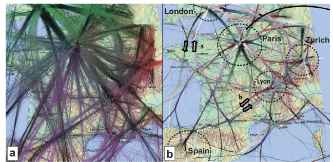
Figure 8: Attribute-driven edge positioning via edge bundling [PHT15]. (a) Raw edges, colored according to directionality. (b) Edges bundled while taking direction into account. © 2015 IEEE, reprinted with permission.
