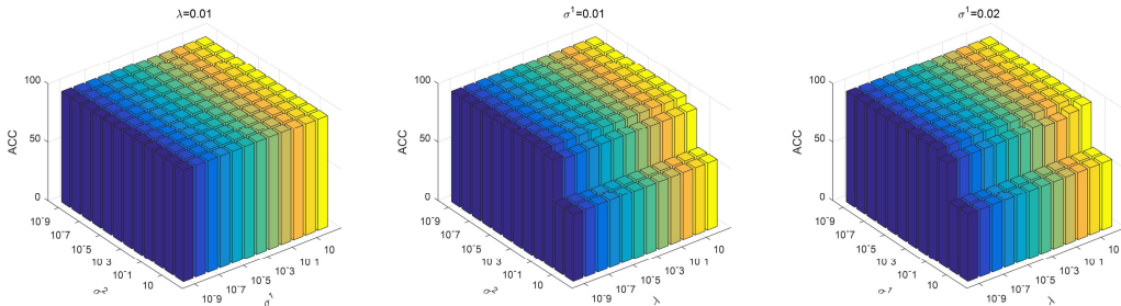
Figure 7. Accuracy of AD vs. NC classification with respect to different parameter values in ADNI-2 dataset. We fix one parameter to 0.01 respectively and vary the other two in the range of \{10^{-9}, 10^{-8}, \dots, 10^2\} . The X-axis and Y-axis represent the diverse value of parameters and the Z-axis represents the classification accuracy for AD diagnosis.
