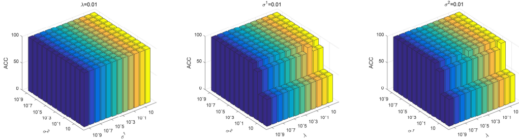
Figure 6. Accuracy of AD vs. NC classification with respect to different parameter values in ADNI-1 dataset. We fix one parameter to 0.01 respectively and vary the other two in the range of \{10^{-9}, 10^{-8}, \dots, 10^2\} . The X-axis and Y-axis represent the diverse value of parameters and the Z-axis represents the classification accuracy for AD diagnosis.
