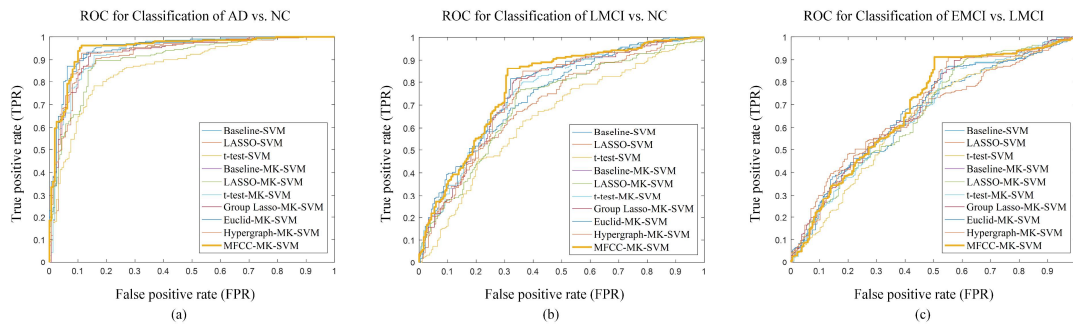
Figure 4. The ROC curves of all comparison methods on ADNI-2: (a) the classification of AD
