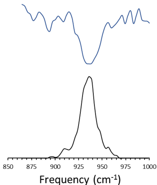
Fig. 1. Comparison of the vibrational action spectra for [\text{UVO}_2(\text{Cl})_3]^- recorded using depletion of precursor ion (top trace) and by photodissociation involving elimination of Cl radical to generate [\text{UVO}_2(\text{Cl})_2]^- .
