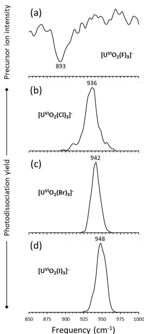
Fig. 2. Comparison of vibrational action spectra for (a) [\text{UVO}_2(\text{F})_3]^- , (b) [\text{UVO}_2(\text{Cl})_3]^- , (c) [\text{UVO}_2(\text{Br})_3]^- and (d) [\text{UVO}_2(\text{I})_3]^- using irradiation in a quadrupole ion trap instrument.
