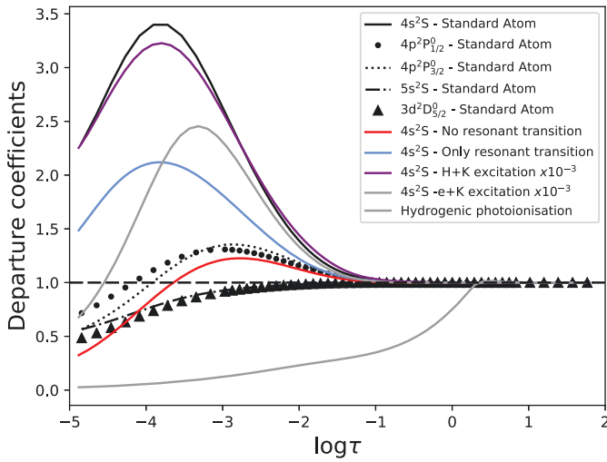
Fig. 3. Departure coefficients for the low-excited K I levels in the solar atmosphere.
