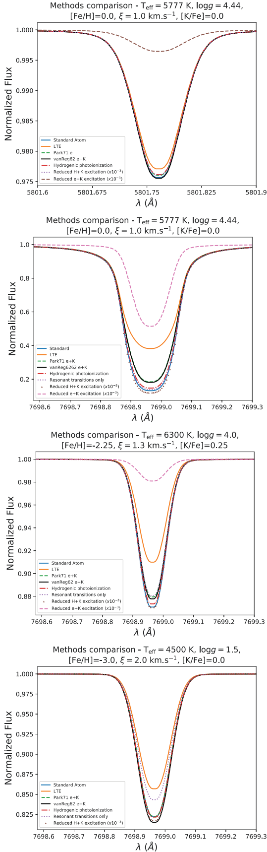
Fig. 4. First and second panels: comparison between the synthetic spectral lines using different collisional recipes for the 5801 and 7698 \text{\AA} lines in the 1D solar atmosphere. Third and fourth panels: the same but for a 1D metal-poor atmosphere (HD 84937) and a giant star 1D atmosphere, respectively.
