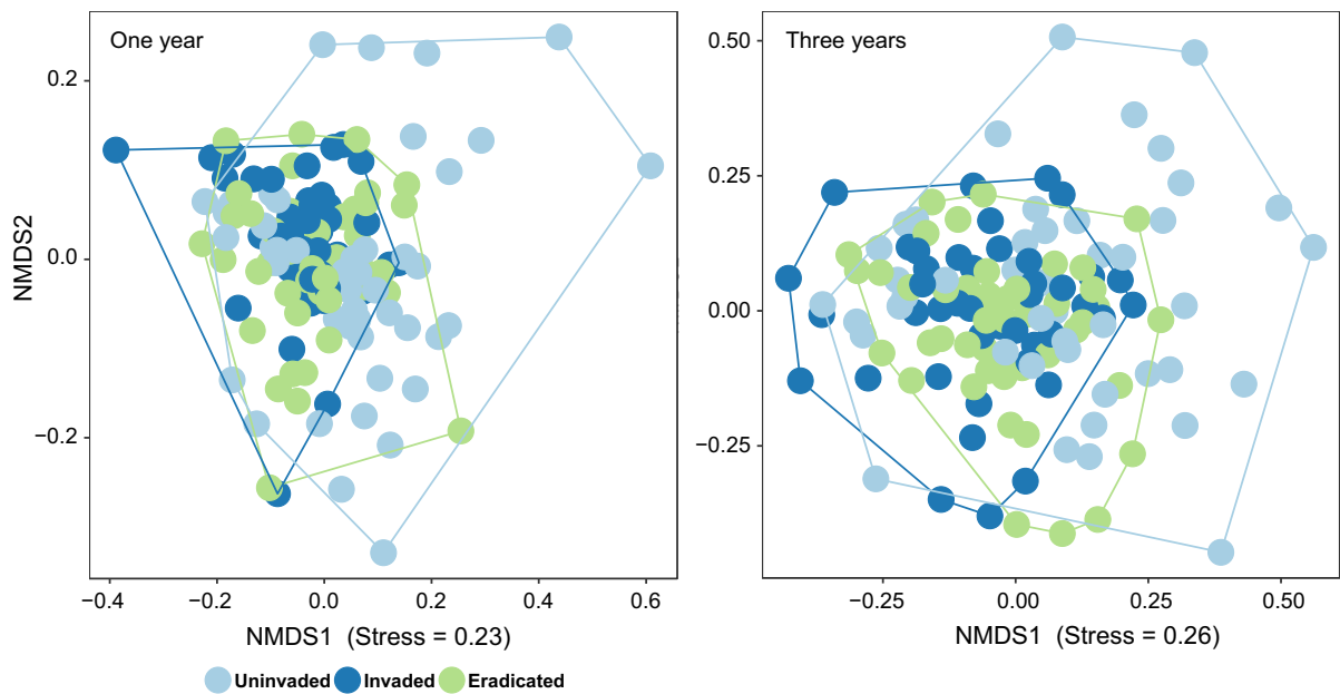
Fig. 1 Fungal community composition 1 and 3 years after garlic mustard eradication. Points represent the Bray–Curtis dissimilarity across sites, with the range in dissimilarity across invasion statuses shown using polygons
