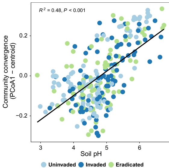
Fig. 3 Community convergence in relation to soil pH across invasion statuses. Positive values indicate that communities are converging towards a common composition (decreasing beta diversity) while negative values indicate that communities are diverging away from a common composition (increasing beta diversity)
