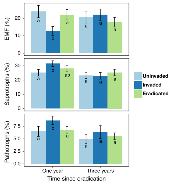
Fig. 2 The relative abundance of fungal functional guilds 1 and 3 years after garlic mustard eradication. Bars represent the mean and error bars are the standard error. Different lowercase letters are significantly different
