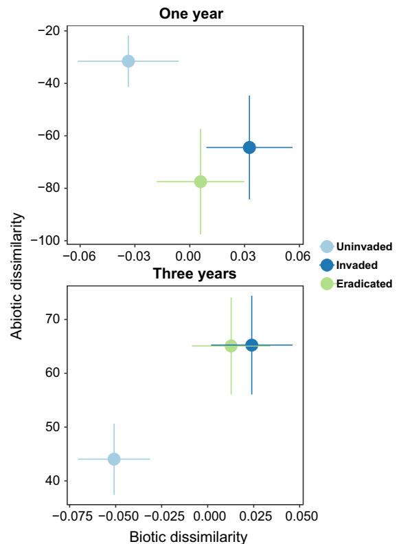
Fig. 4 Overall dissimilarity in the fungal (biotic) and edaphic (abiotic) components of soils one and three years after eradication in the reference uninvaded, invaded, and eradicated plots. Points represent the centroid of fungal community composition (Bray-Curtis) in principle correspondence analysis (axis 1) and edaphic property composition (Euclidean) in principle correspondence analysis (axis 1) and error bars are the standard deviation
