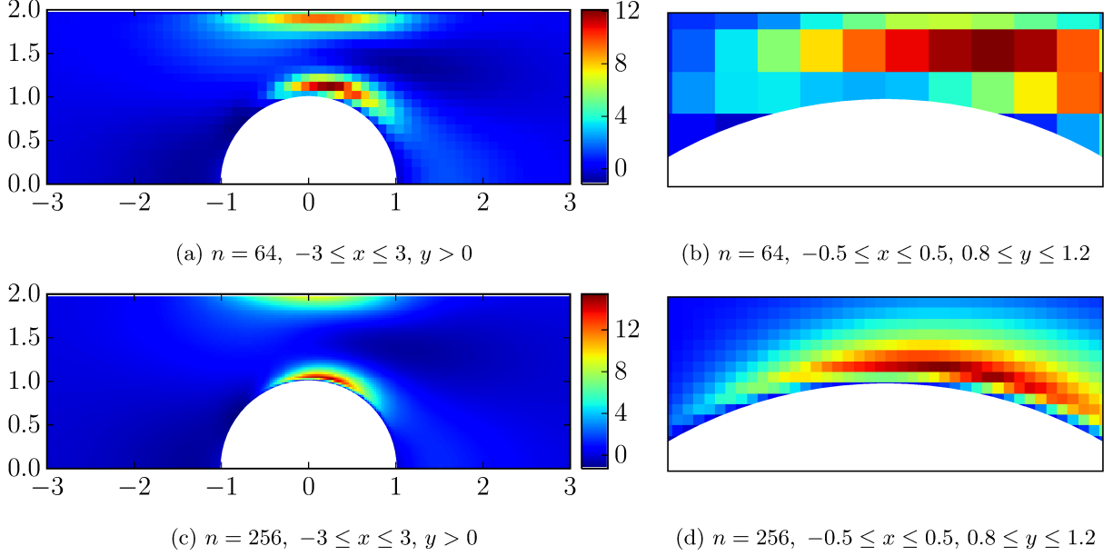
Figure 2: The xx -component of the polymeric stress \tau_P for the Stokes Oldroyd-B flow around the cylinder problem, computed by the Immersed Boundary method, with n_y = 64 (a, b) and n_y = 256 (c, d), and Weissenberg number Wi = 0.1 . In (a, c), the stress \tau_{P_{xx}} is shown in the upper half of the channel ( y > 0 ), for -3 \leq x \leq 3 . In (b, d), a zoom near the cylinder wall is shown, with -0.5 \leq x \leq 0.5 and 0.8 \leq y \leq 1.2 .
