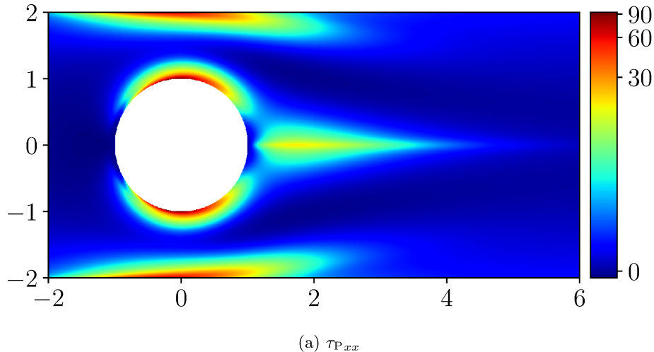
Figure 6: Figure 6a shows the xx -component of the extra polymeric stress \tau_P for the Stokes Oldroyd-B flow around the cylinder problem, computed by the IBSE method, with n_y = 1024 and Weissenberg number Wi = 0.7 . Note that the color scale has been logged, and that the flow domain is longer than is shown.
