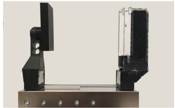
Fig. 10: The Weiss Force Measurement Finger attached to the left finger of the Weiss hand and the sensor with rounded configuration attached to the right finger. The sensor's outputs are measured as the gripper width is varied.
