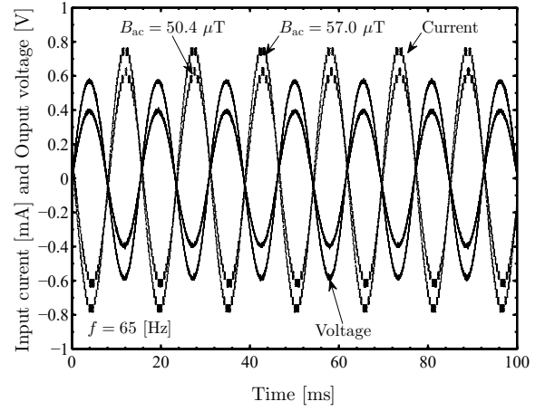
Figure 5: Waveforms of the current input to the Helmholtz coil and the output voltage V_L induced in a load resistance of R_L = 200 \text{ k}\Omega in two cases B_{ac} = 50.4 \text{ }\mu\text{T} and 57.0 \text{ }\mu\text{T} .
