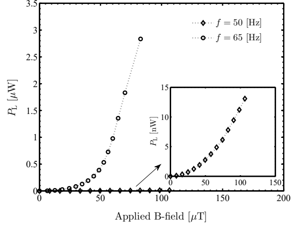
Figure 7: \mathbf{B} -field responses of the transferred power with fixed driving frequencies and R_L = 200 \text{ k}\Omega .
