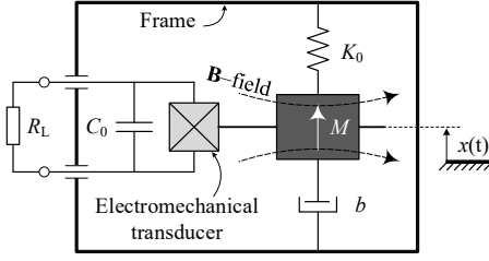
Figure 1: A generic model of an electromechanical-based WPTS.
