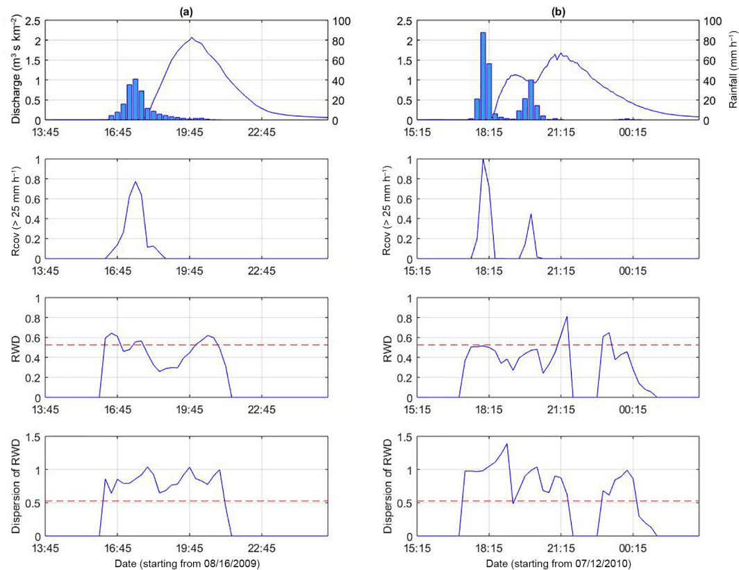
Figure 5. Time series of basin-average rainfall, flow, portion of basin covered by high-intensity rainfall ( > 25 \text{ mm h}^{-1} ), normalized rainfall-weighted flow distance (RWD) and RWD dispersion in Lower LSugar, for two events that occurred on 16 August 2009 (a) and 12 July 2010 (b).
