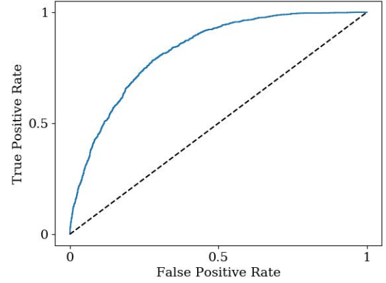
Figure 2: ROC curve of described parameters: AUC of 81.37%
