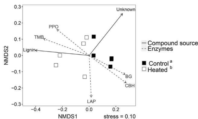
Fig. 2. NMDS ordination of chemical compound relative abundance generated by py-GC/MS analysis of plant litter decomposed for two years under experimental warming. Data were log + 1 transformed prior to analysis. Points represent the chemical composition of different samples. Vectors represent the correlations of relative abundance of compound source classes (solid lines; unknown compound class refers to compounds that were detected by py-GC/MS but which are of unknown origin) or enzyme activities (dashed lines) with the underlying chemical compound matrix. Only significant correlations are plotted. Enzyme abbreviations: BG = beta-glucosidase; CBH = cellobiohydrolase; PPO = polyphenol oxidase (L-DOPA); TMB = peroxidase; LAP = leucine aminopeptidase.
