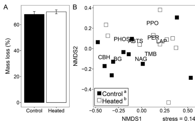
Fig. 1. Mass loss (A) and NMDS ordination of enzyme activities (B). Enzyme activities were relativized by the maximum value for each enzyme before ordination. Superscript letters in panel B figure legend indicate significant differences between treatments. Abbreviations in panel B: BG = beta-glucosidase; CBH = cellobiohydrolase; PPO = polyphenol oxidase (L-DOPA); PER = gross oxidase-peroxidase (L-DOPA + H 2 O 2 ); ABTS = polyphenol oxidase; TMB = peroxidase; LAP = leucine aminopeptidase; NAG = N-acetyl glucosaminidase; PHOS = acid phosphatase.
