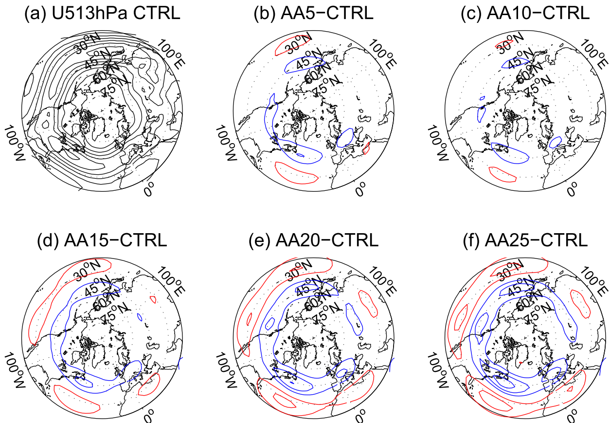
FIG. 5. As in Fig. 2, but for zonal wind over NH at 513 hPa. The CI is 5 \text{ m s}^{-1} in (a), 2 \text{ m s}^{-1} in (b), and 5 \text{ m s}^{-1} in (c)–(f).
