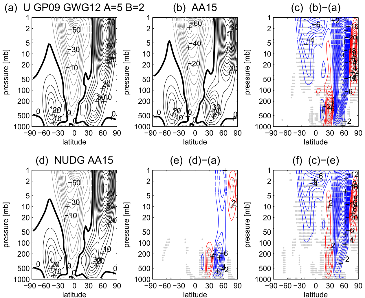
FIG. 12. As in Fig. 9, but using the GP09 model version with a tropospheric jet located near 42°N.
