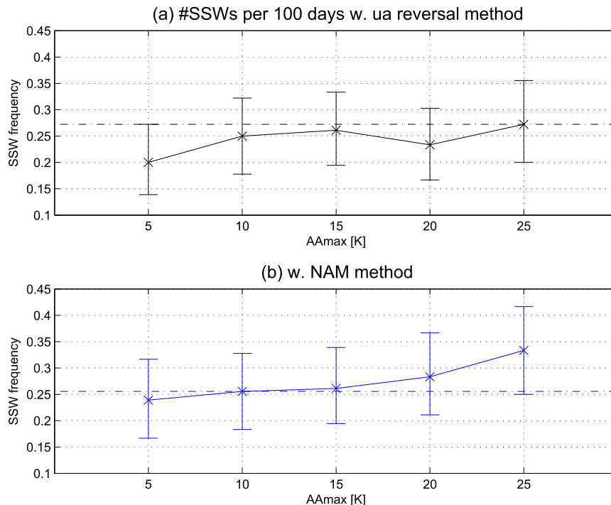
FIG. 6. SSW frequency in CTRL and AA experiments using (a) the standard method with reversal of westerly wind and (b) the NAM method. The results are plotted in dashed-dotted lines for CTRL and crosses for the AA experiments with error bars showing the 2.5th and 97.5th percentiles using the bootstrapping method.
