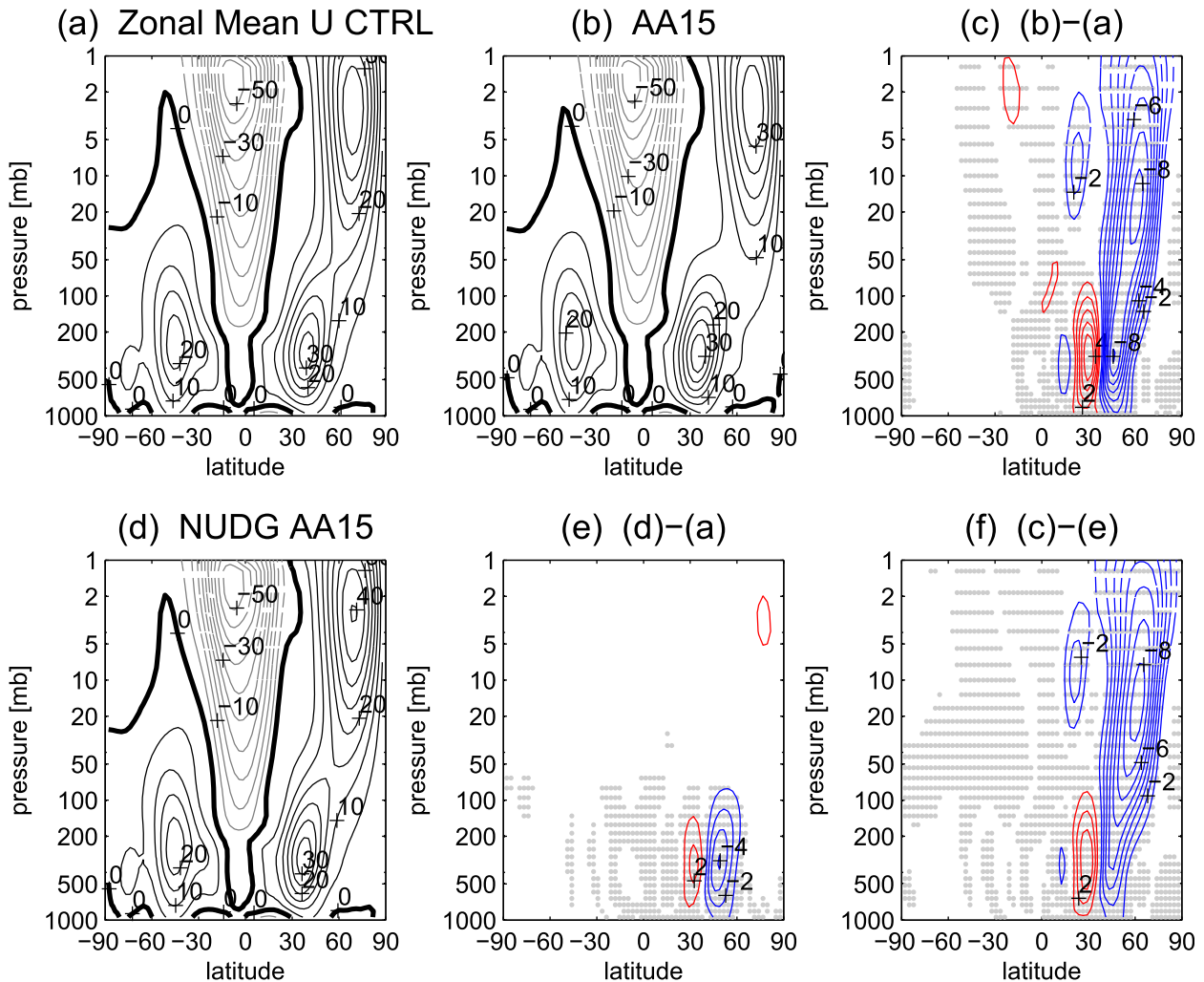
FIG. 9. Zonal-mean zonal wind in (a) CTRL and (b) AA15 experiments and (c) their difference. (d) Zonal-mean zonal wind in the NUDG AA15 experiment and (e) its change compared to CTRL (can be considered as the response via the troposphere only). (f) The difference in zonal wind response between (c) and (e) (which can be considered as the response via the stratospheric pathway only). Note that (a) and (c) are similar to Figs. 2a and 2d, respectively. The CI is 5 \text{ m s}^{-1} in (a), (b), (d) and 1 \text{ m s}^{-1} in (c), (e), (f).
