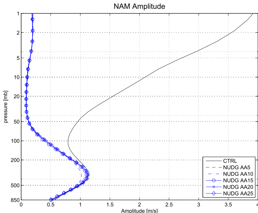
FIG. 8. NAM amplitude as a function of pressure levels in CTRL and NUDG AA experiments. See text for details in the calculation of NAM amplitude.
