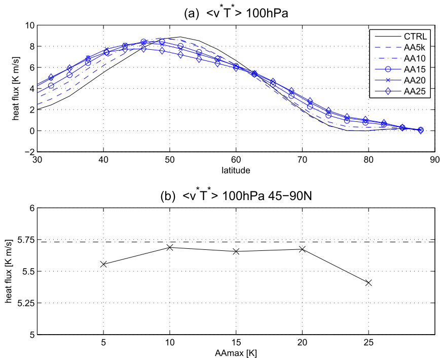
FIG. 7. Eddy meridional heat flux (a) at 100 hPa and (b) averaged poleward of 45°N in CTRL and AA experiments.
