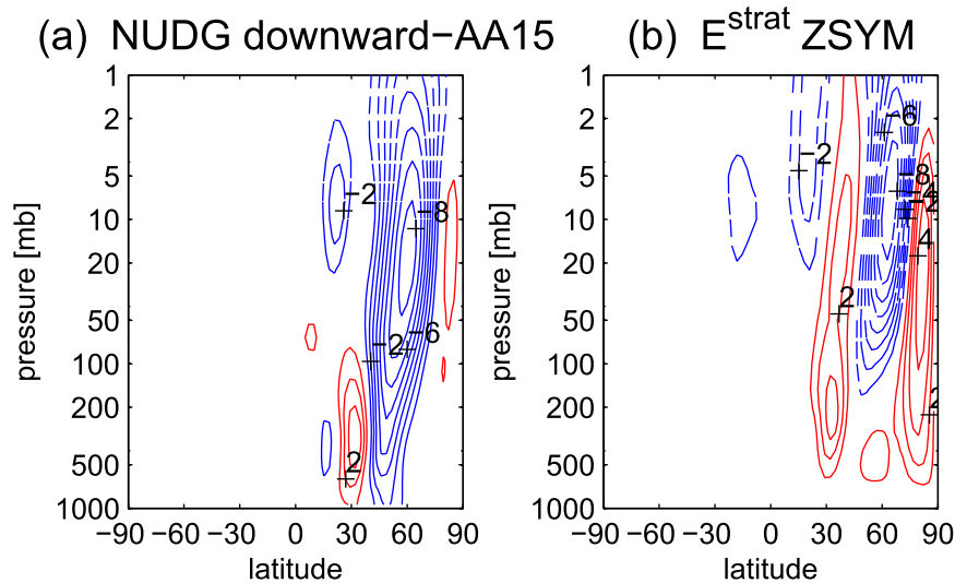
FIG. 10. Zonal-mean zonal wind response (a) in NUDG downward-AA15 experiment and (b) in ZSYM E^{\text{strat}} . The CI is 1 \text{ m s}^{-1} .
