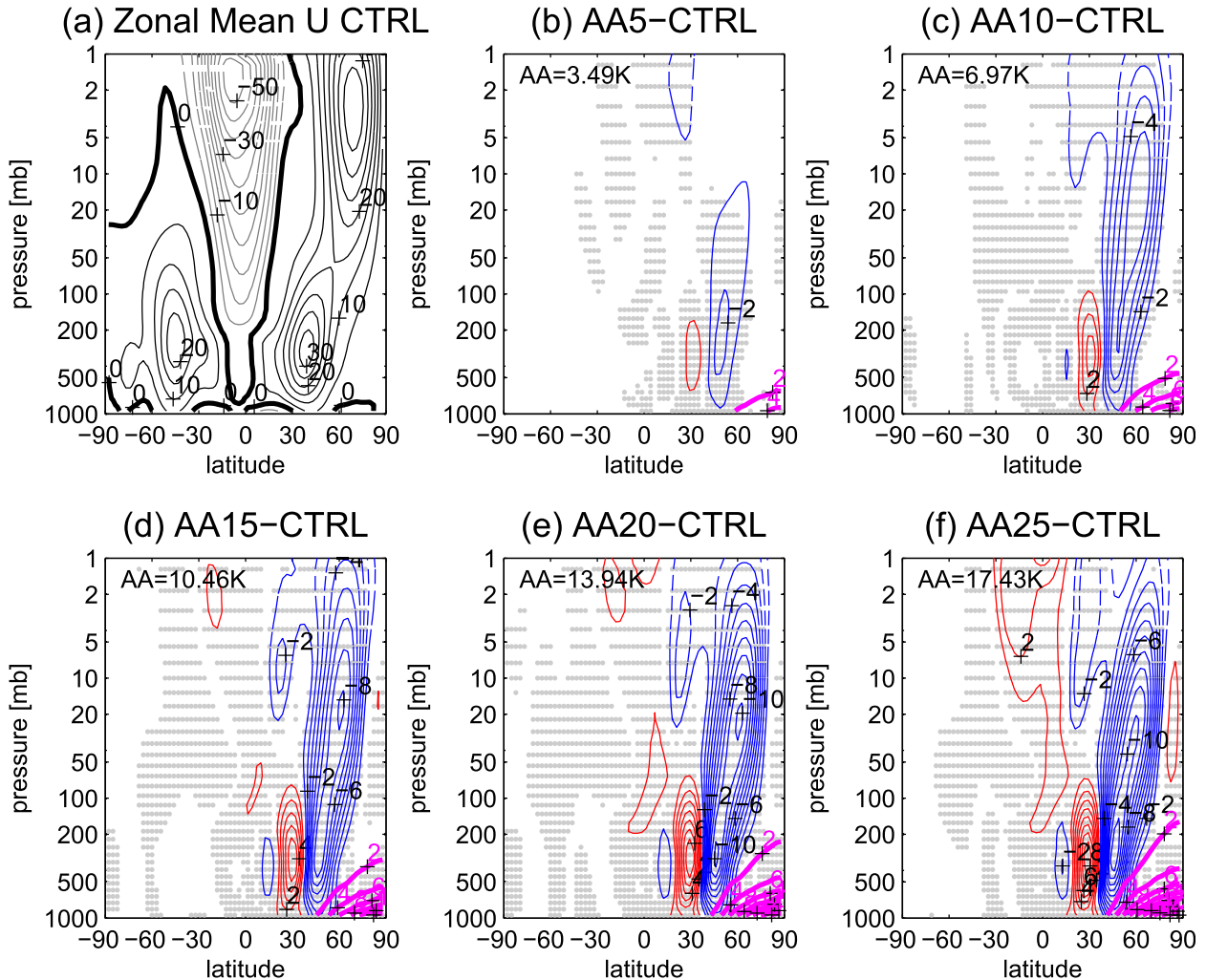
FIG. 2. (a) Zonal-mean zonal wind in CTRL (with the SFK10 model version); response of zonal-mean zonal wind in the (b) AA5, (c) AA10, (d) AA15, (e) AA20, and (f) AA25 experiments. The contour interval (CI) is 5 \text{ m s}^{-1} in (a), with black contours for positive values, gray contours for negative values, and thick black contours for zero values. The CI is 1 \text{ m s}^{-1} in (b)–(f), with red for positive and blue for negative. The magenta contours plot T_{\text{eq}}^{\text{AA}} as in Eq. (2) with CI = 2 K. The numbers in the top-left corner of (b)–(f) indicate the magnitude of AA, which is the near-surface temperature increase poleward of 67.5^\circ\text{N} in T_{\text{eq}}^{\text{AA}} . Statistically significant responses, at the 95% level, are dotted.
