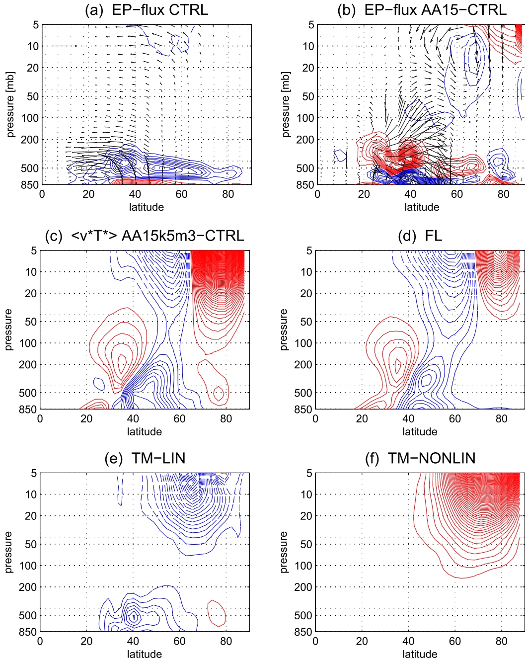
FIG. 4. (a) EP flux in CTRL and (b) its response to AA15. The EP flux vectors are scaled according to Eq. (3.13) of Edmon et al. (1980), and the horizontal arrow scale ( 10^{15} \text{ m}^3 ) is indicated in the top-left corner of (a). The EP flux vectors in (b) are scaled by a factor of 20. The CI is 1 \text{ m s}^{-1} \text{ day}^{-1} in (a) and 0.2 \text{ m s}^{-1} \text{ day}^{-1} in (b) with red contours for positive values and blue for negative. (c) Response in eddy meridional heat flux and its decomposition into the (d) high-frequency wave FL term, (e) time-mean linear term ( \text{TM}_{\text{LIN}} ), and (f) time-mean nonlinear term ( \text{TM}_{\text{NONLIN}} ). The CI is 0.5 \text{ K m s}^{-1} in (c)–(f).
