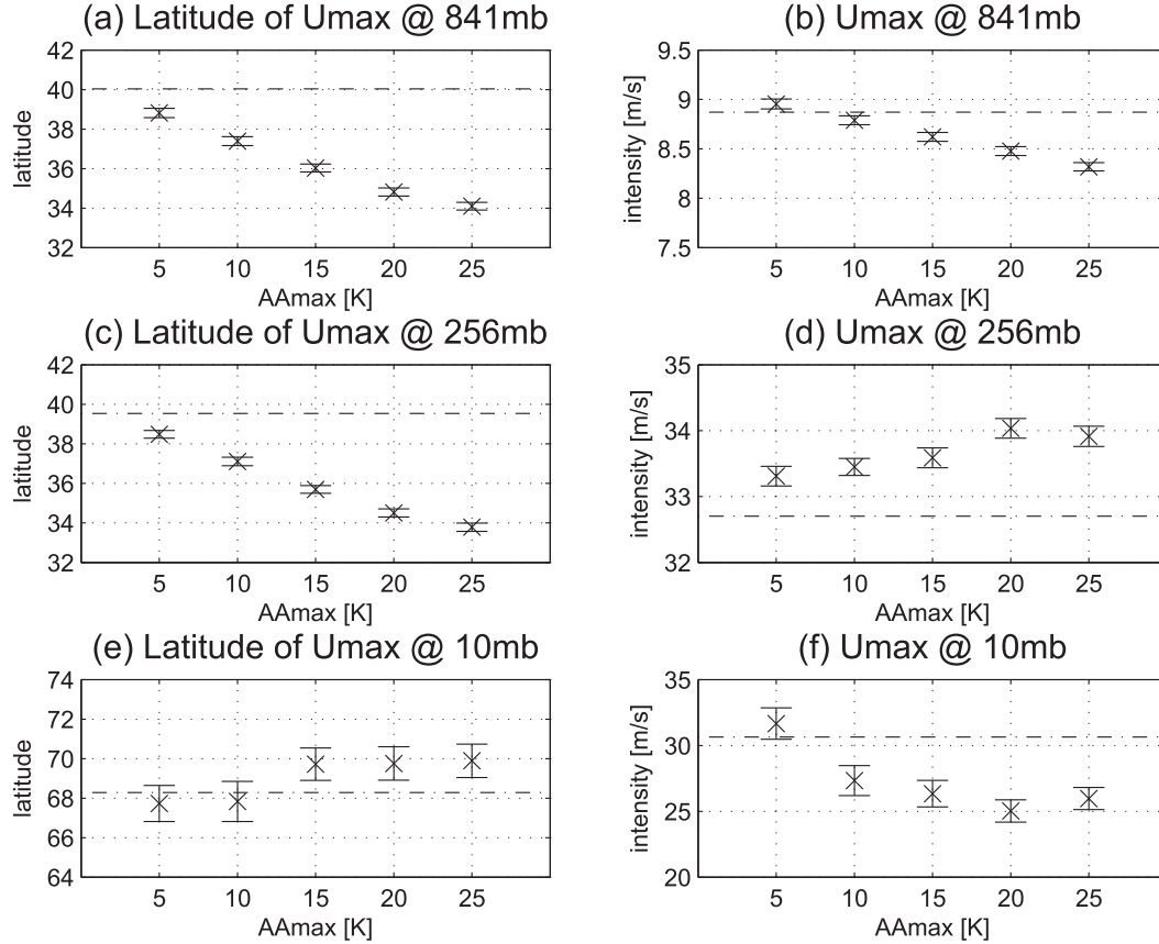
FIG. 3. (left) Latitude and (right) intensity of maximal zonal-mean zonal wind for CTRL and AA experiments at (a),(b) 841; (c),(d) 256; and (e),(f) 10 hPa. The results are plotted in dashed-dotted lines for CTRL and crosses for the AA experiments with error bars showing two standard deviations.
