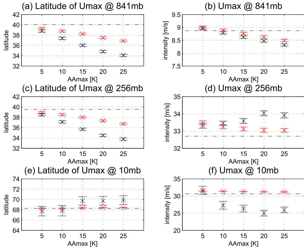
FIG. 11. As in Fig. 3, but including the results from NUDG experiments, plotted with red crosses and error bars.
