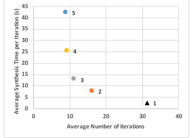
Figure 4: Experimental results with more pairs of scenarios ranked per iteration.
