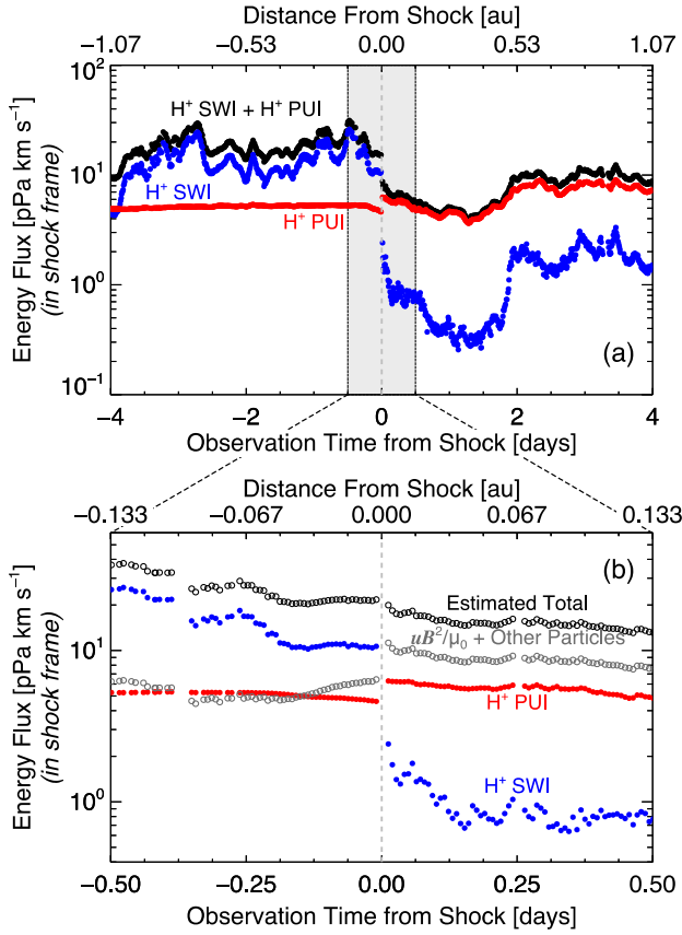
FIG. 3. (a) Energy flux for H^+ SWIs (blue), H^+ PUIs (red), and their total (black) in the shock frame. We perform 1 h boxcar smoothing over SW density and speed. PUI data are interpolated to the SWI measurement resolution. (b) Energy flux close to the shock. We also show the estimated energy flux contribution from the magnetic field, alphas, He^+ PUIs, H^+ PUI tail, electrons, and energetic particles (gray open circles), and the estimated total (black open circles). Note that the PUI density and temperature are assumed constant in panel (b) using the two PUI data points closest to the shock (horizontal lines in Fig. 1 right before and after the shock).
