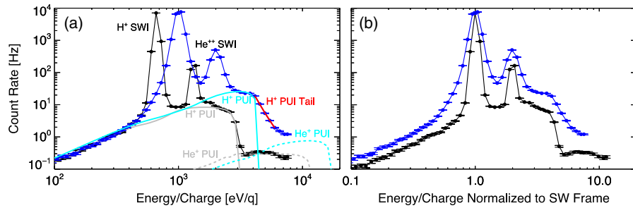
FIG. 4. (a) SWAP day-averaged count rates in the spacecraft frame before (black) and after (blue) the shock (see Fig. 1). Fits to the H^+ PUIs before and after the shock are shown in gray and cyan, respectively. A fit to the H^+ PUI tail after the shock is shown in red. Models of the He^+ PUIs are shown as dashed lines. (b) Data are normalized to the SW frame.
