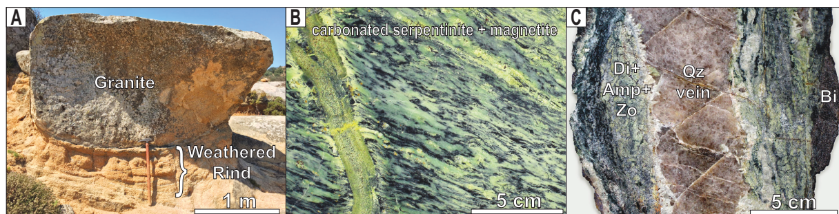
FIGURE 2. Photographs of carbonation/decarbonation processes. (a) Silicate weathering: granite exposed at Earth's surface undergoes spheroidal weathering resulting in discrete boulders with thick physical and chemical weathering rinds. Volax, Tinos Island, Greece. (b) High-temperature carbonation: yellow Ni-bearing calcite has precipitated in an ultramafic rock of the Maltby Lakes Metavolcanics, Connecticut. (c) Infiltration-driven decarbonation: quartz vein (center; Qz) with diopside (Di) + amphibole (Amp) + zoisite (Zo) selvages cutting biotite-bearing metacarbonate rock (dark margins; Bi) of the Wepawaug Schist, Connecticut. Prograde reactions, such as \text{Phlogopite} + 3 \text{ Calcite} + 6 \text{ Quartz} = 3 \text{ Diopside} + \text{K-feldspar} + 3 \text{ CO}_2 + \text{H}_2\text{O} , generated significant \text{CO}_2 (Ague 2003; Stewart and Ague 2018).
