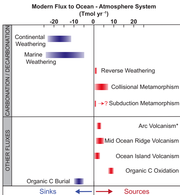
FIGURE 5. Estimates of modern \text{CO}_2 fluxes to the ocean-atmosphere system. Error bars indicate a range of possible values, not necessarily a normal distribution. * Note that the flux from Arc Volcanism includes some contribution from decarbonation of subducting slabs; in fact, slab decarbonation could account for the vast majority of the arc volcanic flux. Arc magmas may also incorporate partially melted carbonate lithologies and drive contact metamorphism in adjacent rocks.
