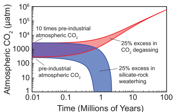
FIGURE 6. Predicted atmospheric \text{CO}_2 concentrations in an Earth system where \text{CO}_2 sources and sinks do not balance, modified after Berner and Caldeira (1997). Regardless of starting \text{CO}_2 concentration, a 25% excess in \text{CO}_2 degassing (red curves) or a 25% excess in silicate weathering (blue curves) result in a run-away atmospheric composition within \sim 1 million years.
