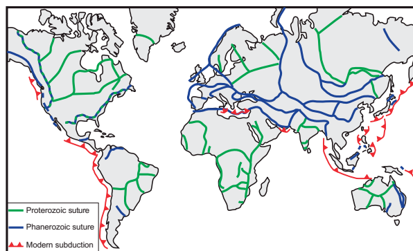
FIGURE 3. Global map indicating the locations of modern subduction (red lines with carets), and ancient sutures formed in the Phanerozoic (blue) and Proterozoic (green). Sutures that were active during both eons are dashed blue and green. Modified after Orme (2015) and Burke et al. (1977).
