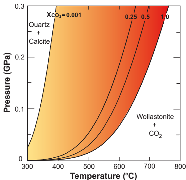
FIGURE 4. Pressure-Temperature diagram showing the stability of the assemblage calcite + quartz relative to wollastonite + \text{CO}_2 . Conditions of this reaction are calculated for equilibrium between minerals and fluid of differing \text{CO}_2 content ( X_{\text{CO}_2} is the mole fraction of \text{CO}_2 in fluid). Calculations made using the program Theriak-Domino (de Capitani and Petrakakis 2010) with the Holland and Powell (1998) database.
