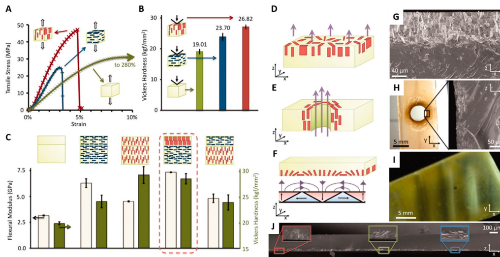
Figure 3. (A) Improvement in tensile strength for polymer with 20 vol.% Al 2 O 3 platelets parallel with applied force (red) vs. perpendicular (blue) and non-reinforced (green) samples (B) Increased hardness for reinforced resins with 10 vol.% Al 2 O 3 platelets parallel to the applied load versus perpendicular and non-reinforced samples (C) Flexural modulus and out-of-plane hardness of bilayer rectangular samples with different combinations of reinforcement orientation in samples produced using field-assisted, non-AM methods (D) Particles aligned along z-axis due to applied field (G) SEM of particles aligned in z-axis (E) Reinforcing particles concentrated around a hole (H) SEM of particles distributed around hole in part (F) Graduated particle alignment achieved by refrigerator magnets (I) Topological ripples formed in a polymer substrate due to particle alignment (J) SEM image of Mohawk-like structure in layer [74].
