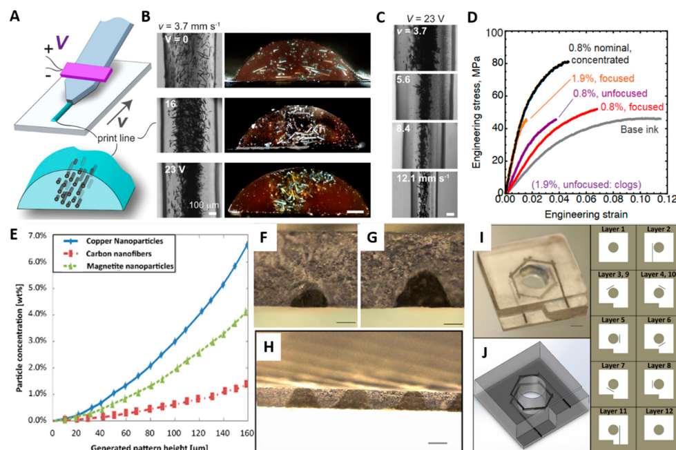
Figure 6. (A) Schematic of a microfluidic print nozzle with a coupled piezoelectric actuator driven at a peak-to-peak voltage (V), with deposition speed controlled by the substrate velocity (V). (B,C) Print line microstructures for a constant deposition speed of 3.7 mm s -1 and increasing excitation voltage from 0 to 23 V in plain view and cross-section (D) Mechanical characterization of SiC/epoxy inks for tensile tests of the base ink material (epoxy, no fibers) as well as inks with 0.8 vol.% SiC fibers for unfocused and focused condition [86] (E) Relationship between reinforcement concentration and pattern height for different materials (F) sample cross-section with 50 μm reinforcement height (G) 100 μm reinforcement height in a 200 μm sample (H) 100 μm reinforcement height in a 100 μm sample (I) 12 layer embedded electromagnetic coil pattern surrounding magnetic core cavity (J) 3D schematic of electromagnet pattern in UV resin [87].
