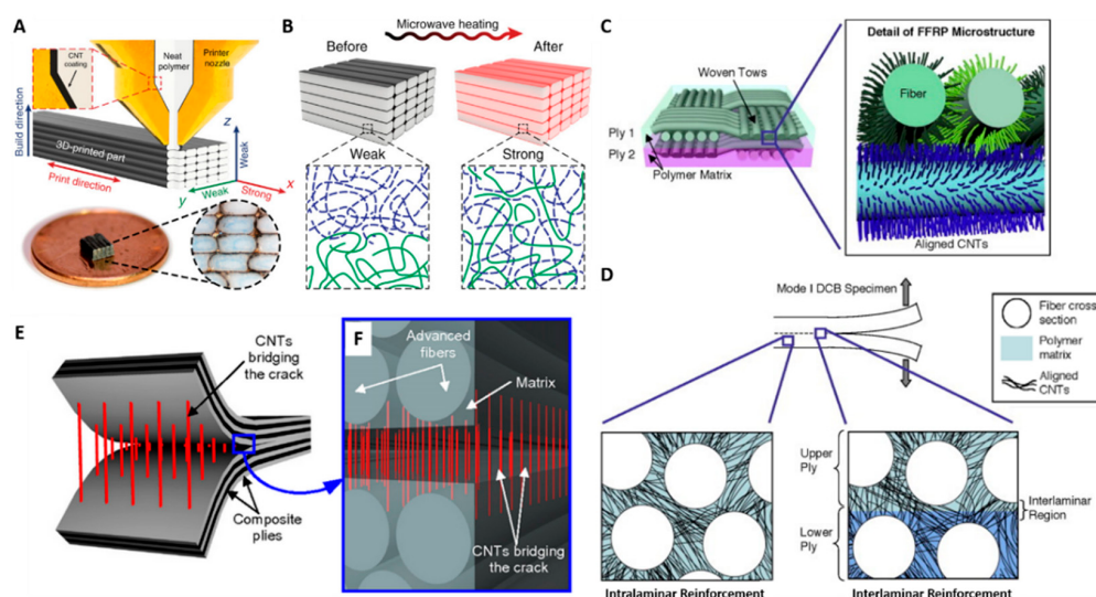
Figure 2. (A,B) Essentium's process of filling voids formed during extrusion with the use of CNT-coated thermoplastic filament [83], (C) Radially aligned CNTs grown on advanced fiber cloth, (D) CNT intralaminar and interlaminar reinforcement [80], (E,F) use of aligned CNT forests to strengthen interlaminar region in composite laminates [67].
