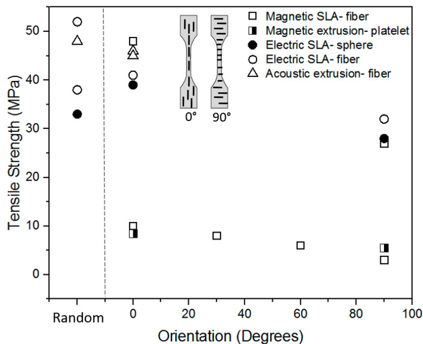
Figure 7. Tensile strength of various composites manufacturing using SLA or extrusion AM with applied magnetic, electric, and acoustic fields [53,58,59,71,82,107,113].
