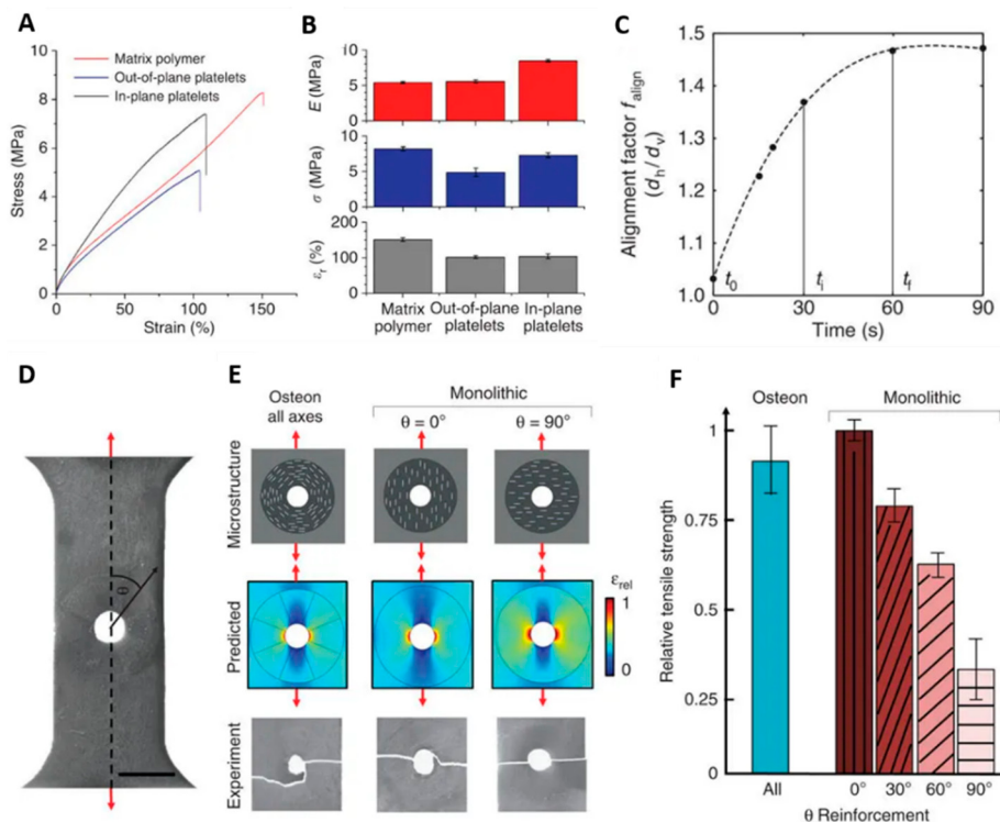
Figure 4. (A) Stress-strain curves of magnetically aligned platelets in different orientations (B) elastic modulus ( E ), strength ( \sigma ) and strain-at-rupture ( \epsilon_r ) of printed samples (C) alignment dynamics of platelets in the presence of a rotating magnetic field and the increase in the degree of platelet alignment as a function of time [53] (D) Samples with circular defects are 3D magnetic printed with programmable reinforcement architectures including “osteon-inspired” microstructures with concentric reinforcement orientation and “monolithic” microstructures as shown in (E). (E) “Osteon-inspired” microstructures are predicted to exhibit less relative strain compared with misaligned “monolithic” microstructures. (F) Tensile tests of printed composites with circular defects show that “osteon-inspired” architectures out-perform all but the perfectly aligned “monolithic” sample. As the “osteon-inspired” architecture is symmetric, the load can be applied at any angle relative to the microstructure to obtain similar performance. Scale bar, 5 mm in (D) [59].
