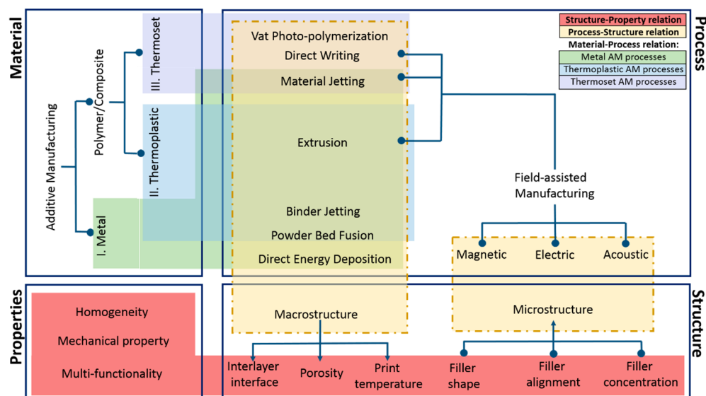
Figure 1. Material-process-structure-property relationship classifying AM processes.
