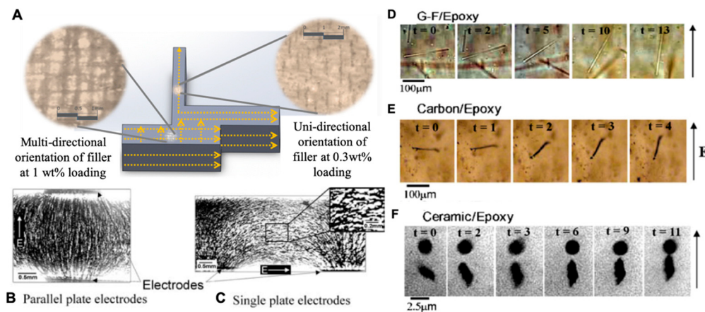
Figure 5. (A) AM part showcasing directionality and unidirectionality of reinforcement in a single component [85] (B) Parallel plate electrodes produce chains oriented through thickness of the material (C) Planar electrodes form in-plane chains [117] (D) Time sequence and orientation of glass fiber in response to an electric field E = 0.7 \text{ kV mm}^{-1} (E) carbon fiber (F) ceramic particles in a liquid epoxy of viscosity 2.5 \text{ Pa.s} [118].
