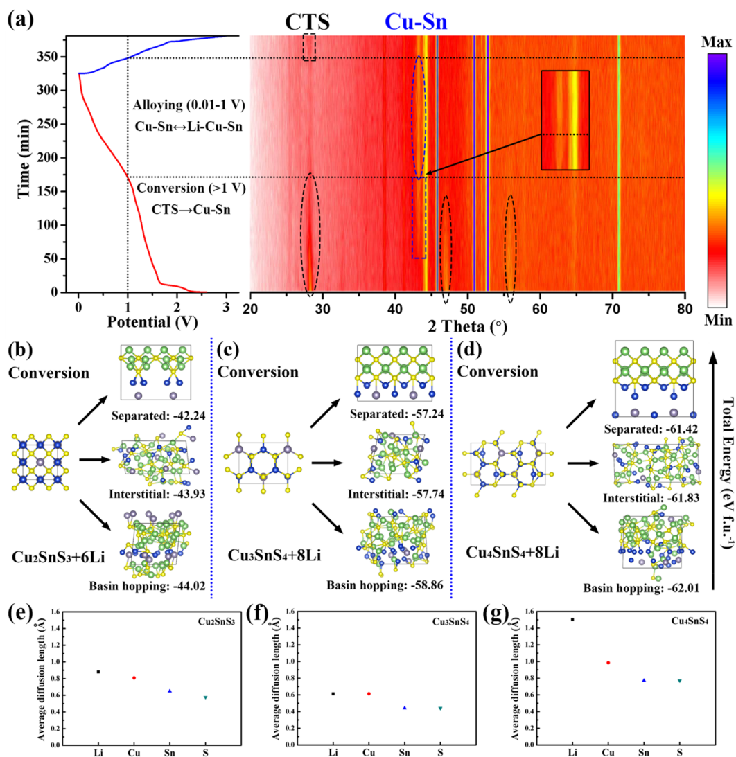
Figure 4. (a) In situ XRD patterns and corresponding charge/discharge curves of CTS/G-414 upon the initial lithiation and delithiation. Calculated atomic structural evolution of (b) \text{Cu}_2\text{SnS}_3 , (c) \text{Cu}_3\text{SnS}_4 , and (d) \text{Cu}_4\text{SnS}_4 upon conversion process by three different algorithms. Average atomic diffusion lengths of Li, Cu, Sn, and S in (e) \text{Cu}_2\text{SnS}_3 , (f) \text{Cu}_3\text{SnS}_4 , and (g) \text{Cu}_4\text{SnS}_4 .
