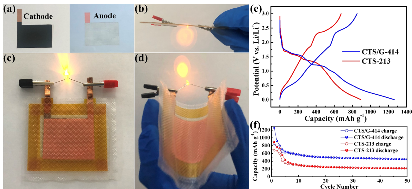
Figure 7. (a) Photographs of CTS/G-414 cathode and lithium-foil anode. (b) Side view, (c) top view, and (d) bending state of the thin and flexible Li-metal batteries when driving light-emitting diodes. (e) Initial charge/discharge curves and (f) cycling performance of the thin and flexible Li-metal batteries using CTS/G-414 and CTS-213 electrodes.
