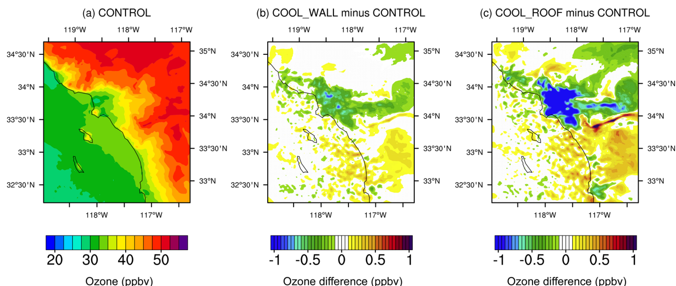
Figure 2. Spatially resolved daily maximum 8-h average (MDA8) ozone concentrations (ppbv) for (a) the CONTROL scenario, and changes relative to CONTROL for scenarios (b) COOL_WALL and (c) COOL_ROOF. Changes that are not statistically distinguishable from zero (see Section 2.4 for details on statistical analysis) in (b) and (c) are dotted. Values are temporally averaged over the period of 00:00 LST on July 3 to 00:00 LST on July 12.
