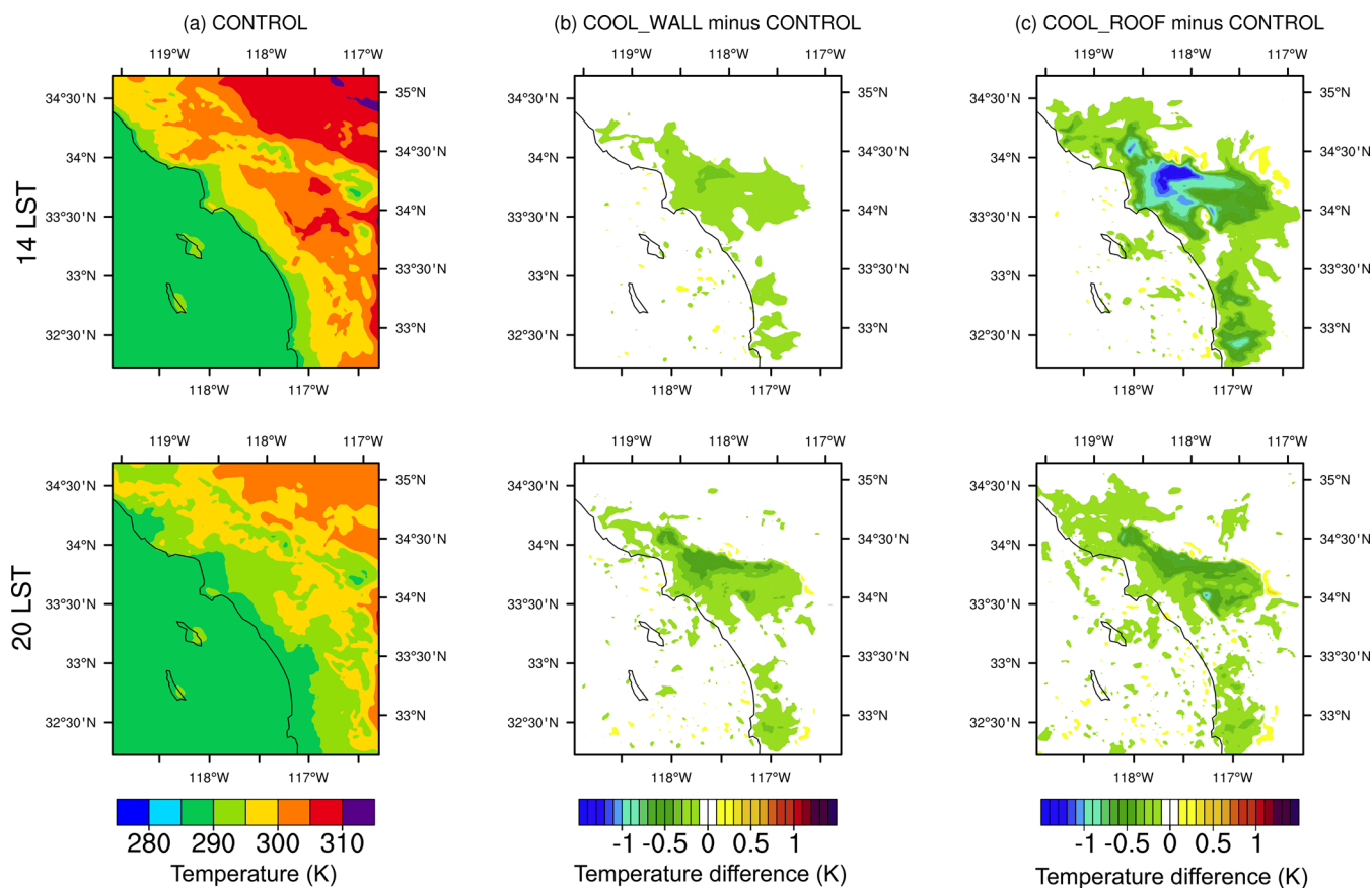
Figure 1. Spatially resolved near-surface air temperatures (K) at 14:00 LST and 20:00 LST for (a) the CONTROL scenario, and the difference relative to CONTROL for (b) COOL_WALL and (c) COOL_ROOF. Values are temporally averaged over the period of 00:00 LST on July 3 to 00:00 LST on July 12.
