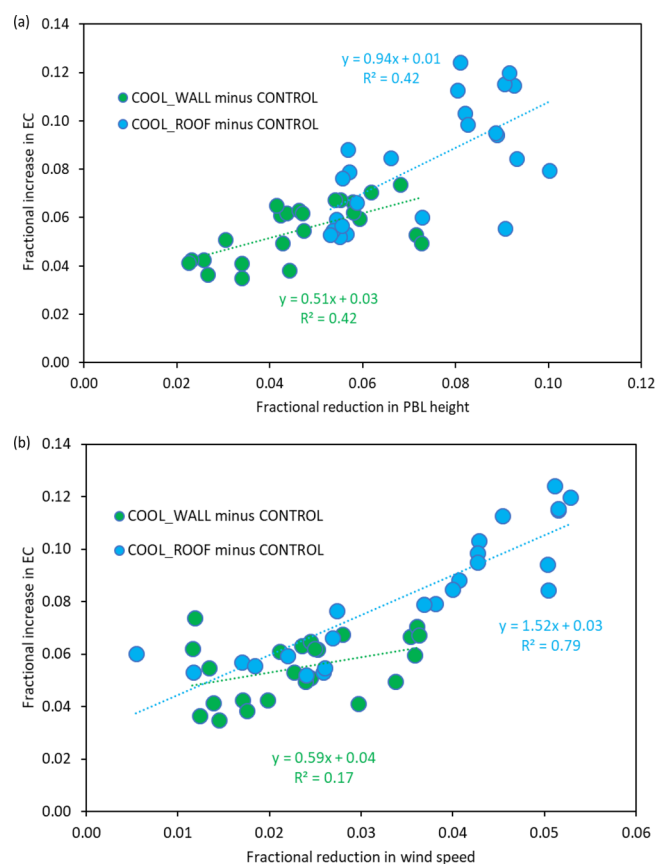
Figure 5. Scatter plots showing fractional increase in EC concentrations induced by cool walls and cool roofs versus (a) fractional reduction in PBL height and (b) fractional reduction in 10-m wind speed. Least-squares linear regressions and corresponding coefficients of determination ( R^2 ) are also shown. Values represent spatial averages in Los Angeles County (i.e., shown in Figure S3c ) for urban grid cells from 00:00 LST on July 3 to 00:00 LST on July 12.
