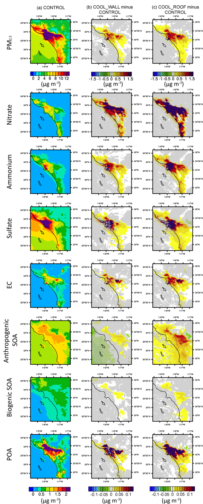
Figure 3. Daily average \text{PM}_{2.5} concentrations ( \mu\text{g m}^{-3} ) by species for CONTROL (left column), as well as the differences for COOL_WALL – CONTROL (middle column) and COOL_ROOF – CONTROL (right column). Differences that are not statistically distinguishable from zero (see Section 2.4 for details on statistical analysis) are shaded in gray (middle and right panel columns). Values are temporally averaged over the period of 00:00 LST on July 3 to 00:00 LST on July 12.
