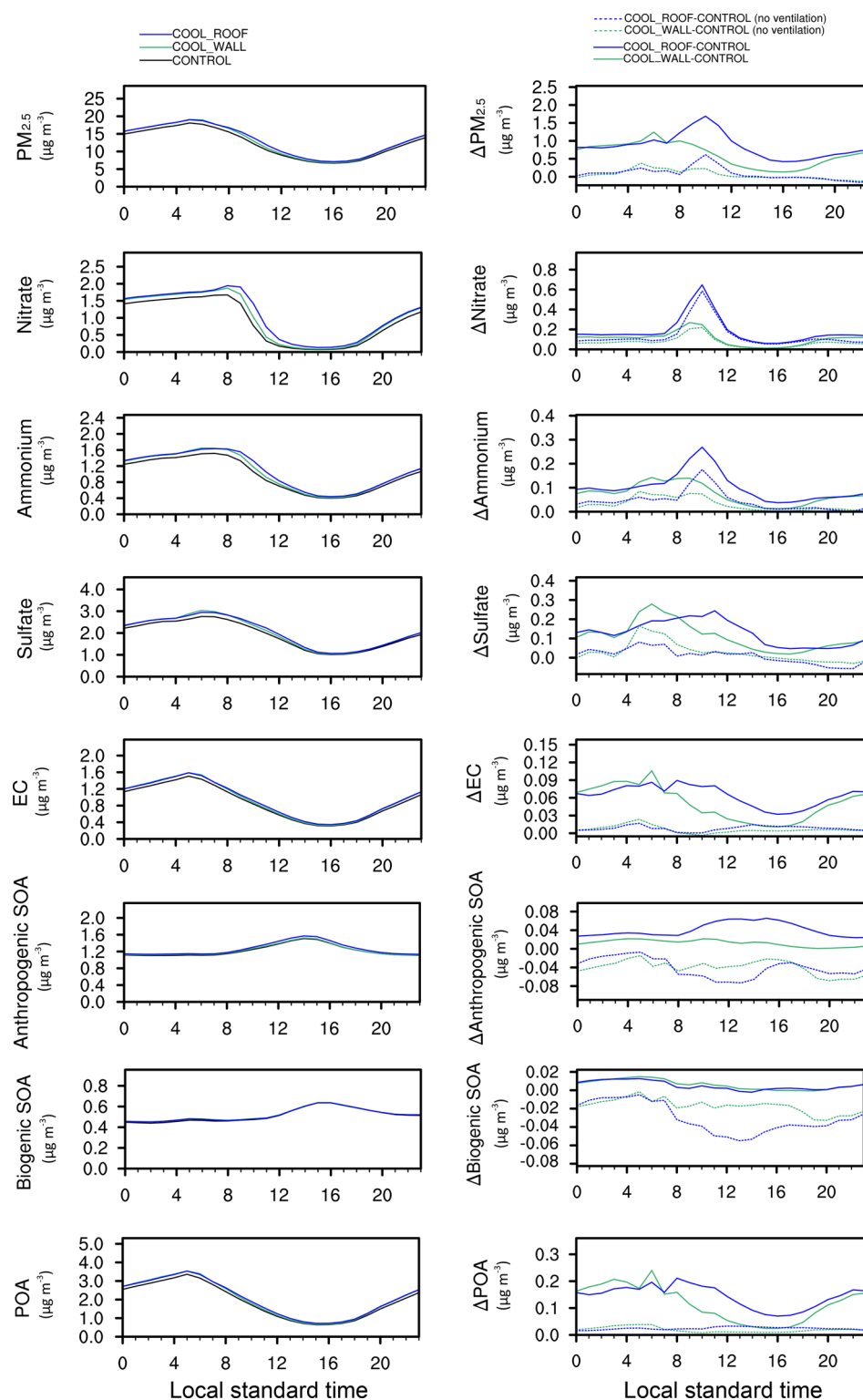
Figure 4. Diurnal cycles of spatially averaged \text{PM}_{2.5} concentrations by species. The left column shows \text{PM}_{2.5} ( \mu\text{g m}^{-3} ) for CONTROL, COOL_WALL, and COOL_ROOF. The right column shows the differences in \text{PM}_{2.5} species for COOL_WALL – CONTROL and COOL_ROOF – CONTROL and the differences if the ventilation effect is excluded. Values represent spatial averages in Los Angeles County (shown in Figure S3c) for urban grid cells from 00:00 LST on July 3 to 00:00 LST on July 12. Note that vertical axis ranges vary for each species.
