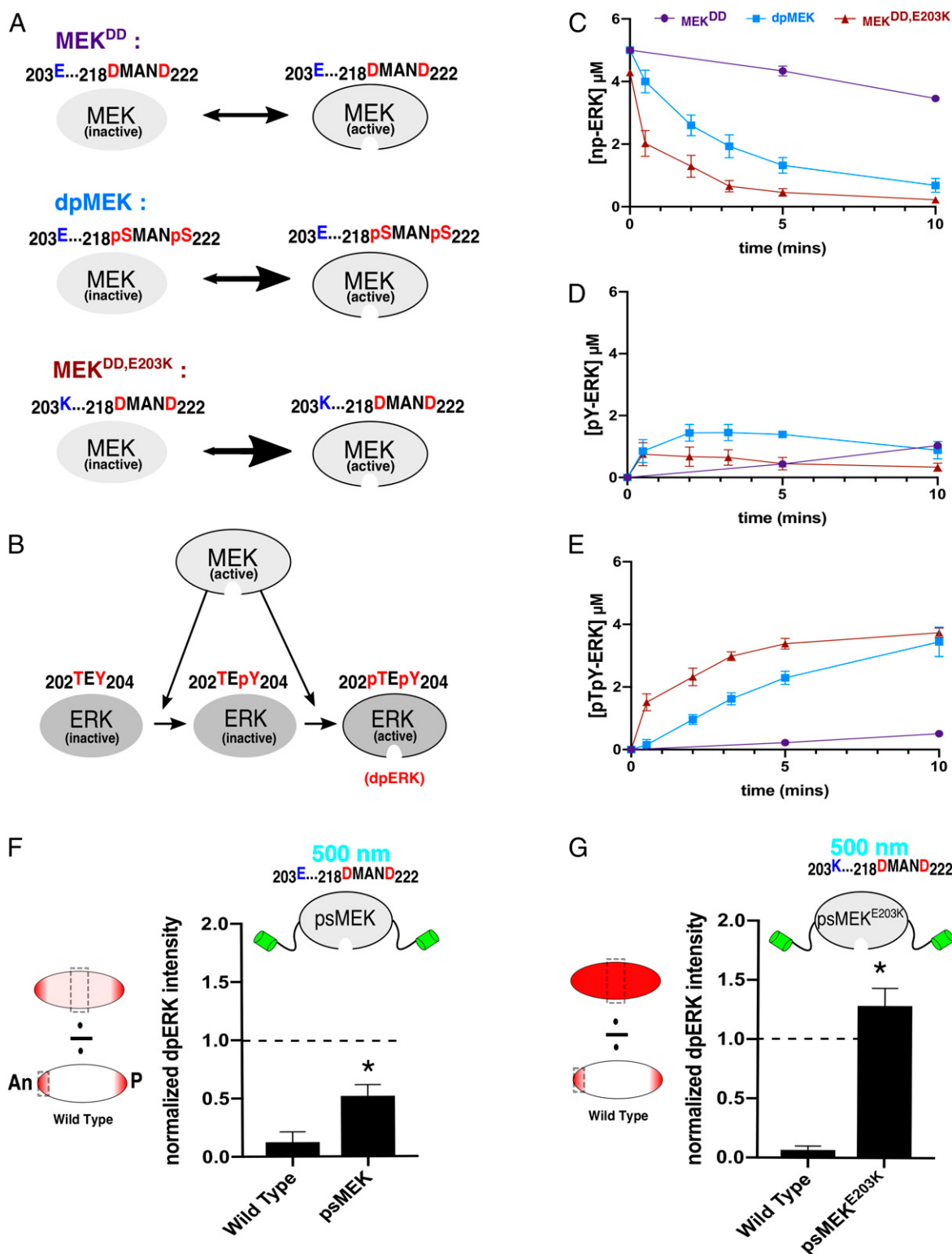
Fig. 2. Enhancing MEK activity with destabilizing mutations. (A) Phosphomimetic MEK (MEK DD ) is predicted to be significantly less active than dpMEK. Destabilizing MEK DD with a distal E203K substitution (blue) creates a different MEK variant (MEK DD,E203K ) that we predict will exhibit increased activity. (B) Active MEK catalyzes dual phosphorylation of ERK. (C) Data from in vitro kinase assays showing kinetics of unphosphorylated ERK (np-ERK) levels in the presence of phosphomimetic (purple, MEK DD ), phosphorylated (light blue, dpMEK), and phosphomimetic MEK with E203K (dark red, MEK DD,E203K ). Data are based on n = 5 for MEK DD and dpMEK and n = 6 for MEK DD,E203K at all time points. (D) Time courses of the monophosphorylated ERK (pY-ERK) levels for 3 different MEK variants. (E) Time courses of the dually phosphorylated ERK (dpERK, pTpY-ERK) levels for 3 different MEK variants. (F) Quantifications of confocal images of immunofluorescence stainings for dpERK in 3-h-old Drosophila embryos. The dpERK intensities in the middle of the embryo (50% embryo length) are presented for WT and psMEK-expressing embryos activated with 500 nm light. All measurements reflect the dpERK levels normalized to the maximum dpERK intensity in the WT control embryos (at the anterior pole). The dashed line drawn at 1.0 represents the maximum dpERK intensity in WT embryos. N_{WT} = 17 and N_{psMEK} = 25 . (G) The same quantifications described for embryos expressing psMEK with an additional E203K mutation, denoted as psMEK E203K . N_{WT} = 18 and N_{psMEK^{E203K}} = 15 . In F and G, *P < 0.05 .
