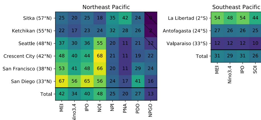
Fig. 4 Percentage of interannual and longer variance accounted for by Pacific climate indices in detrended sea level observations from long, high-quality tide gauges in the East Pacific from 1950 to 2017. Colors map to values; large (small) percentages of variance are highlighted in yellow (purple). Values not significant at the 95% level are marked with a diagonal line. “Total” is the ratio between the sum of (variance accounted for by climate mode at each tide gauge record) and sum of (total sea level variance at each record). A low-pass convolution filter was applied to monthly tide gauge data and climate indices to isolate variability with periods longer than 18 months. The analysis was restricted to the period 1950–2017, which is the period spanned by all climate indices considered here and satisfies the requirement of at least 50 years for separating the influence of climate modes from trends in Pacific sea level (Frankcombe et al. 2015). Tide gauge data are from Permanent Service for Mean Sea Level (Holgate et al. 2013), and detrending is performed using the fitted trend from the regression with the index. See Sect. 3.1.3 of the text for the definitions of climate indices
