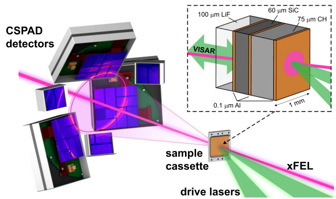
FIG. 1. Schematic of the experimental setup. Samples were mounted in a translatable cassette. The x-ray beam (xFEL) was incident at 15^\circ relative to target normal and the two nanosecond laser arms were oriented at 6^\circ and 25^\circ . Diffracted x rays were recorded on CSPAD detectors. The target package, illustrated on the right, shows the CH ablator, SiC sample, and LiF window. The VISAR was oriented normal to the sample, focused on the LiF-SiC interface.
