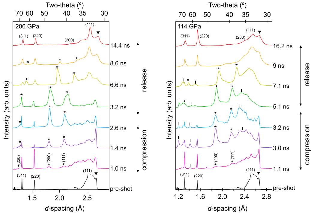
FIG. 3. (a) Integrated x-ray diffraction patterns for time series collected at a peak stress of \sim 206 GPa for polycrystalline 3C starting material. X-ray probe times after the shock enters SiC are listed at the right. B1 peaks are marked with asterisks. Ambient 3C peaks are indexed in the preshot pattern. The feature marked with an inverted triangle at 2.66 Å arises due to stacking fault disorder (Supplemental Material, Fig. S1 [32]). Peaks from the back-transformed 3C phase are indexed in the top pattern. (b) Integrated diffraction patterns for time series collected for a peak stress of \sim 114 GPa. B1 peaks and compressed 3C peaks are marked with asterisks and vertical lines, respectively. X-ray probe times after shock enters SiC are listed at the right.
