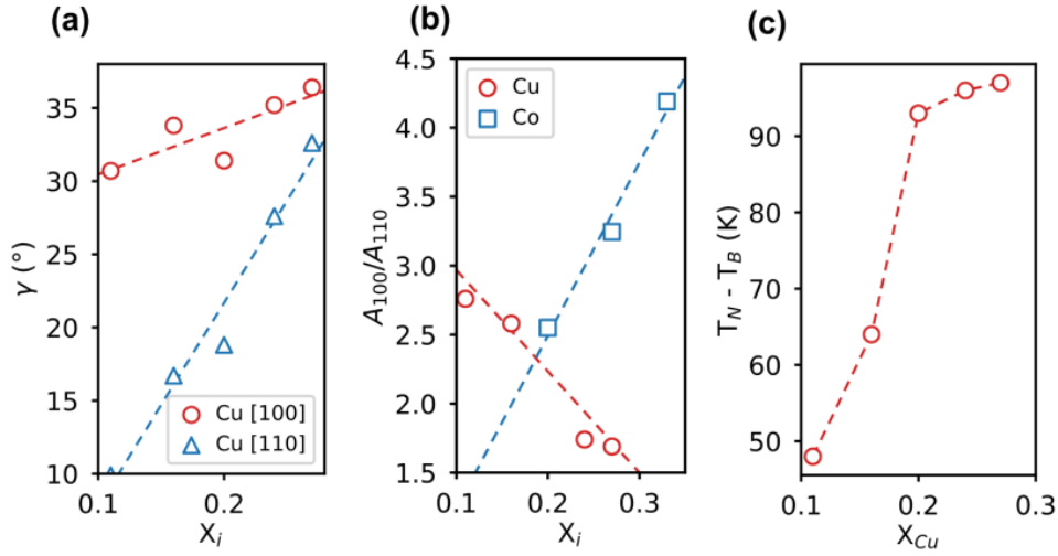
FIG. 5. Anisotropy parameters of the fits to magnetic data. (a) , angle, \gamma , between the applied field and the preferred axis of the spin glass as a function of composition. As the concentration of Cu is increased, the difference between \gamma along the [100] and [110] directions approaches 0, showing that the magnetic lattice is tending toward isotropy with increasing Cu. (b) , Ratio between anisotropy energies for the [100] and [110] directions. As Cu concentration is increased, the ratio approaches 1 and the system tends towards isotropy. As Co concentration is increased, the anisotropy becomes stronger and [110] becomes the preferred easy axis. Dashed lines in each plot are guides to the eye. (c) , Plot of the difference between T_N and T_B reveals the sluggishness of the transition, as a function of Cu concentration, indicating increasing glassiness in the ESO as Cu incorporation is increased.
