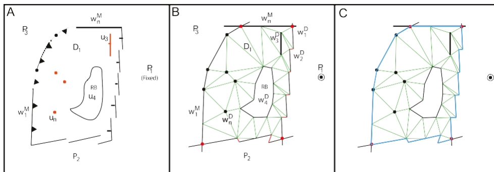
Fig. 1. A. Geological data and concepts used in the reconstruction. B. Their computer representation. C. The continuously closed plate in the computer implementation. In A we have a deformation region ( D_1 ) that is part of plate 1 ( P_1 ). D_1 is bound by a subducting margin on its left hand side and an extending region on its right hand side. The normal faults denote the diffuse boundary between D_1 and P_1 . The top and bottom boundaries mostly accommodate transform motion. Within D_1 there is a collection of deformation points (filled circles), normal faults, and rigid blocks (RB). Points and lines within the interior are shown in orange while those on the boundary are in black. The displacements u_3, u_4, u_n \dots are with respect to fixed plate P_1 . In B we show the computer implementation of the deforming region that is consistent with the concepts of a continuously closing plate (CCP, Gurnis et al., 2012 ). First, the outer boundary of D_1 is a topological closed polygon with the intersection points found at each moment of time. The triangular Delaunay mesh shown in green then represents the continuous deformation within D_1 . Linear interpolation is used to find the velocity and displacements within the mesh. In C the CCP is shown as the blue polygon. (For interpretation of the references to color in this figure legend, the reader is referred to the Web version of this article.)
