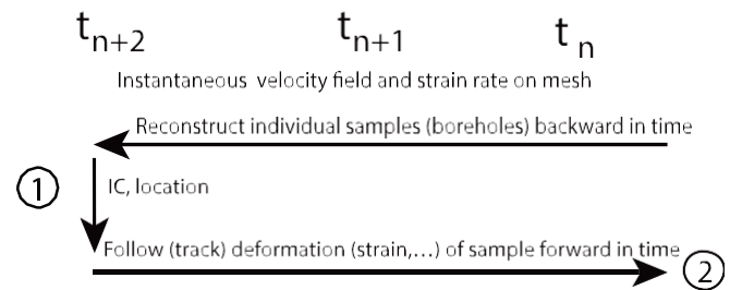
Fig. 2. Flowchart of the time integration of deformation in GPlates 2.1. Step 1 is the backward integration of the position of strain markers to obtain their initial position in the deformation topological network. Step 2 is the forward integration of the finite strain tensor to obtain the deformation history of the strain marker.
