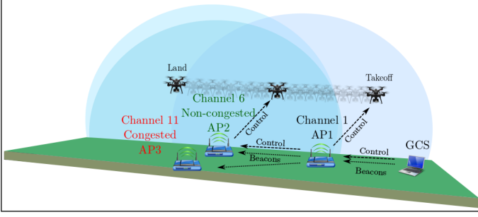
Figure 3. Topology of the experimental setup.
