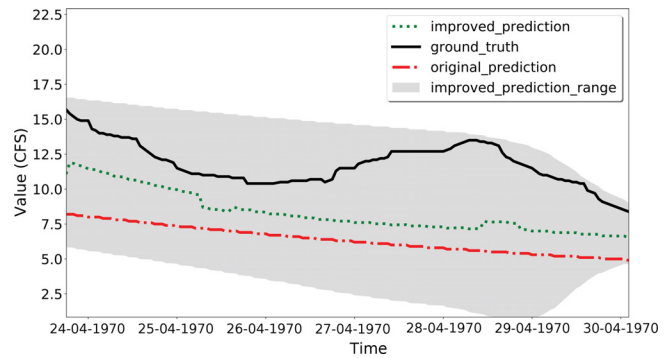
Figure 12. Case Study 2, HEC-HMS PRMS model improvements. The improved predictions are closer to the ground truth than the original predictions.
