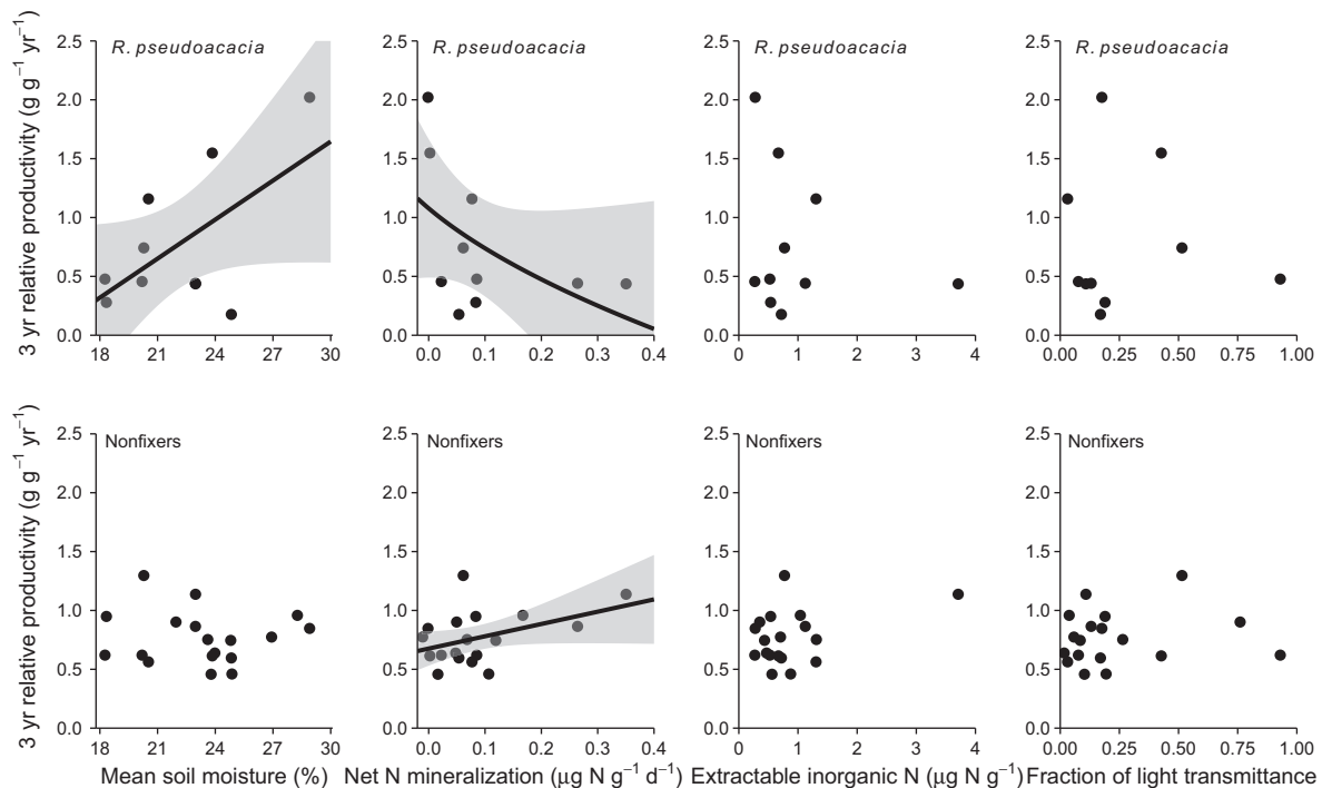
FIG. 1. Aboveground productivity of (top row) Robinia pseudoacacia and (bottom row) nonfixing tree species related to mean growing season soil moisture, net N mineralization, extractable inorganic N and light availability. Aboveground productivity and soil moisture are 3-yr means. Net N mineralization and extractable inorganic N were measured three times during the 2015 growing season using six randomly located 10-cm-deep cores homogenized to one sample per plot. Regression lines with 95% confidence intervals are included when the effect was present in the best model (as selected by BIC).
