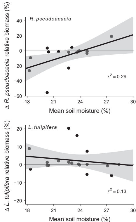
FIG. 2. Change in relative biomass (percent of total tree biomass) of (top) Robinia pseudoacacia and (bottom) Liriodendron tulipifera during years 2 and 3 of the experiment related to mean soil moisture during that period. Lines represent regression fits with 95% confidence intervals and marginal r^2 values (variance explained by mean soil moisture alone).
