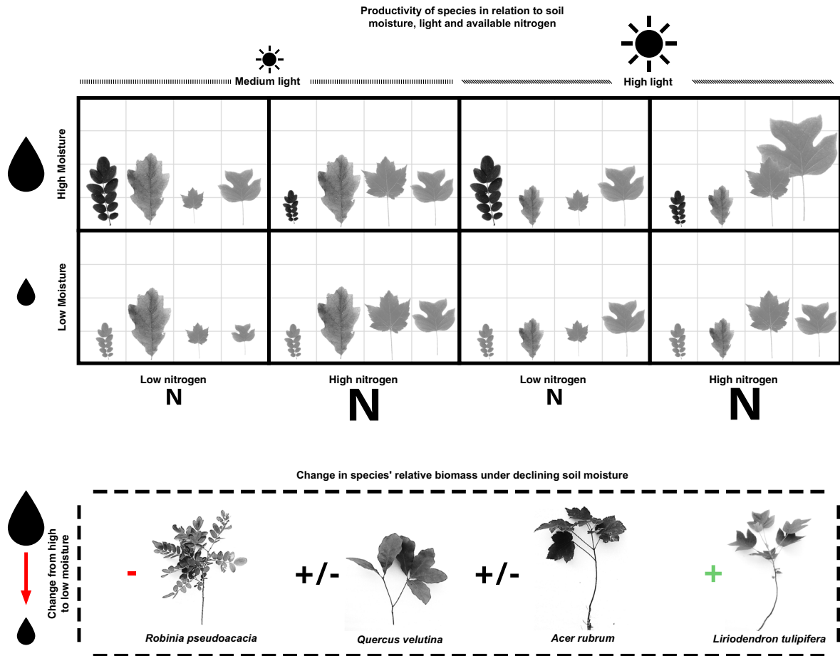
FIG. 6. Synthesis of individual and community-level responses to declining soil moisture. Top panel depicts aboveground productivity and leaf N concentrations for each species in relation to gradients of soil moisture, light, and available nitrogen, where leaf size denotes productivity, and leaf darkness denotes nitrogen concentration. In each box, leaves are ordered from left to right ( Robinia pseudoacacia , Quercus velutina , Acer rubrum , and Liriodendron tulipifera ). Bottom panel depicts change in relative biomass among these four species under declining soil moisture, where + denotes increase, +/- denotes no change, and - denotes decrease.
