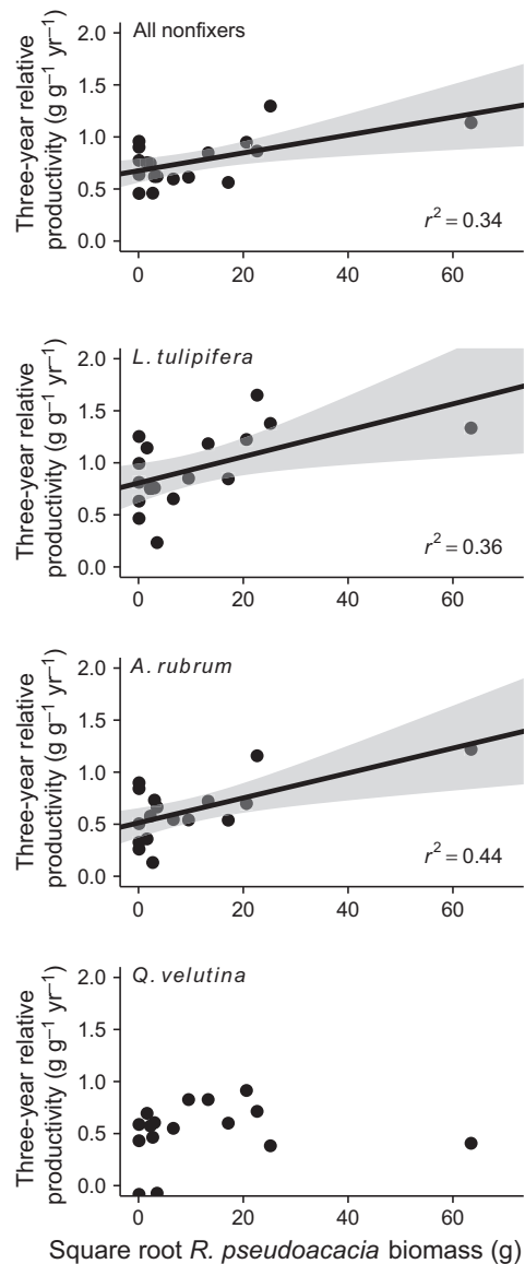
FIG. 4. Robinia pseudoacacia total plot biomass is positively related to relative net aboveground productivity of nonfixing trees (top). When nonfixers were modeled individually, there was a significant relationship for Liriodendron tulipifera and Acer rubrum , but not Quercus velutina . Regression fits with 95% confidence intervals and marginal r^2 values (variance explained by R. pseudoacacia biomass alone) are included for significant relationships. All relationships remain significant if the highest biomass plot is removed.
