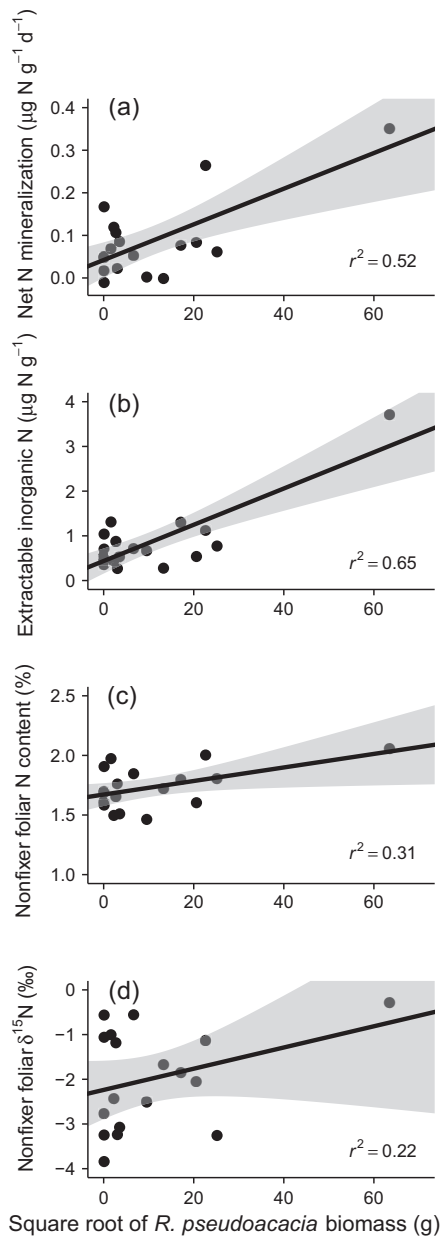
FIG. 3. Robinia pseudoacacia total plot biomass is positively related to (a) net N mineralization rate, (b) extractable inorganic N, (c) foliar N concentration of nonfixing trees, and (d) foliar \delta^{15}\text{N} of nonfixing trees. Values for nonfixing trees represent the mean of the three individual species' mean responses. Biomass of R. pseudoacacia refers to total plot biomass in year 2, the midpoint of the study. Regression fits with 95% confidence intervals and marginal r^2 values (variance explained by R. pseudoacacia biomass alone) are included for significant relationships. All relationships become nonsignificant if the highest biomass plot is removed.
