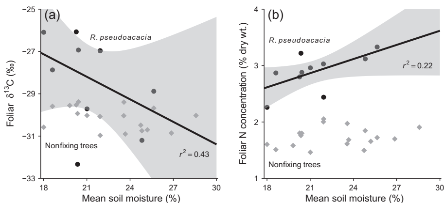
FIG. 5. Changes in \delta^{13}\text{C} and foliar N concentration with soil moisture. (a) Foliar \delta^{13}\text{C} of Robinia pseudoacacia , a measurement of water-use efficiency, increases with declining soil moisture, but there is no effect for nonfixing trees. (b) Foliar N increases with increasing moisture for R. pseudoacacia (circles and solid line), but not nonfixing trees (diamonds). Values for nonfixing trees represent the mean of the three individual species' mean responses. Soil moisture, foliar N and \delta^{13}\text{C} measurements are from the 2015 growing season. Regression fits with 95% confidence intervals and marginal r^2 values (variance explained by mean soil moisture alone) are included for significant relationships.
